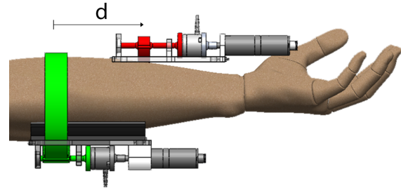
Fig. 3. 3D CAD Model of the stretch and squeeze modules used in this work. Absolute thresholds for the squeeze cue were investigated in the presence of interfering squeeze cues that varied in amplitude and distance from the stretch cue. The distance d represents the distance between the two cues applied
