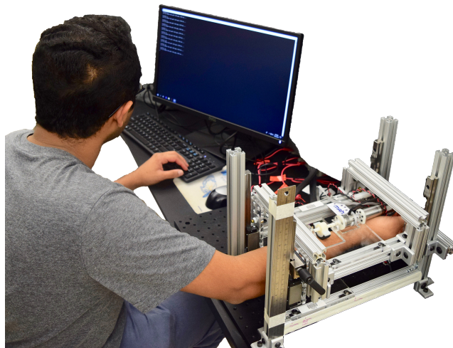
Fig. 1. Experimental setup. In this experiment, participants placed arm in the experimental AIMS testbed, and haptic test cues were applied. The participant answers prompts on the computer monitor regarding detectability of multi-sensory haptic cues delivered to the forearm via the AIMS Testbed. During experimentation, the participant's view of the setup was blocked and the participant wore headphones to isolate them from auditory stimuli.
