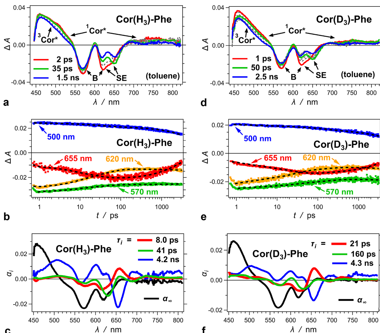
Fig. 3 Transient-absorption dynamics of Cor(H 3 )-Phe and Cor(D 3 )-Phe for toluene media; \lambda_{ex} =400 nm; pulse width=50 fs. a, d TA spectra showing the absorption features of 1 Cor* and 3 Cor*, as well as the ground-state bleach (B) and the stimulated emission (SE). For clarity, only the spectra at picosecond (1–2 ps), tens of picosecond (35–50 ps), and nanosecond (1–3 ns) times are displayed in color. Additional TA spectra at intermediate timepoints are depicted in the background with gray dashed lines. b, e TA kinetic traces recorded at 500 nm, where 1 Cor* and 3 Cor* absorb; 570 nm, where the B is
