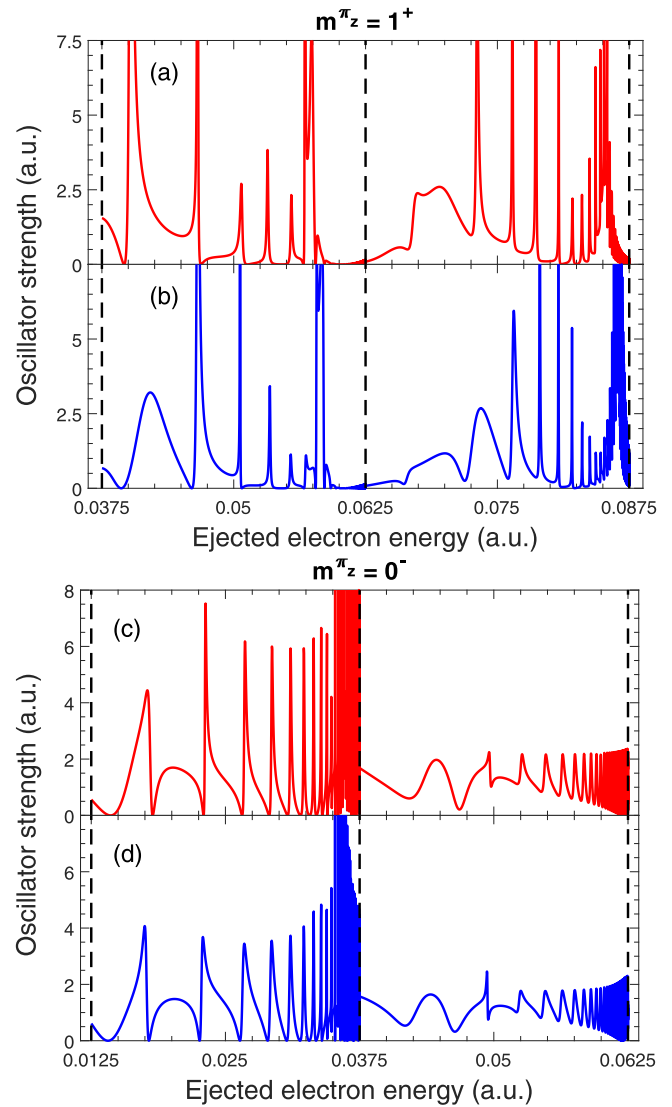
FIG. 6. Same as Fig. 4, but with \gamma = 0.025 a.u.
