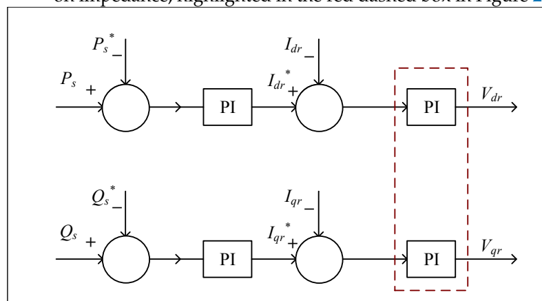
Figure 2. RSC control loops: stator real power ( top loop), and stator reactive power ( bottom loop). Reference values labeled with *.
