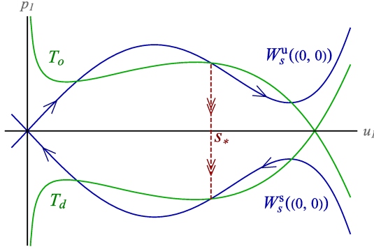
Fig. 2. A schematic representation of the reduced slow flow on \mathcal{M}_0 . The slow stable and unstable manifolds \mathcal{W}_s^{u,s}((0,0)) are indicated in blue, the take-off and touchdown curves T_o and T_d are indicated in green. The jump through the fast field at a transversal intersection of \mathcal{W}_s^u((0,0)) and T_o for u_1 = s_* is indicated in red
