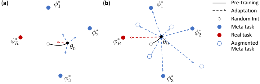
Fig. 2. Comparison of (a) transfer learning and (b) task-augmented meta-learning. (a) After pre-training on very few number of meta tasks, the model is pulled closer to the meta tasks and may be far from the real task. (b) By creating pseudo meta tasks to pre-train the meta-learning model, it gains the ability of adapting to the new tasks with only one gradient step updating.
