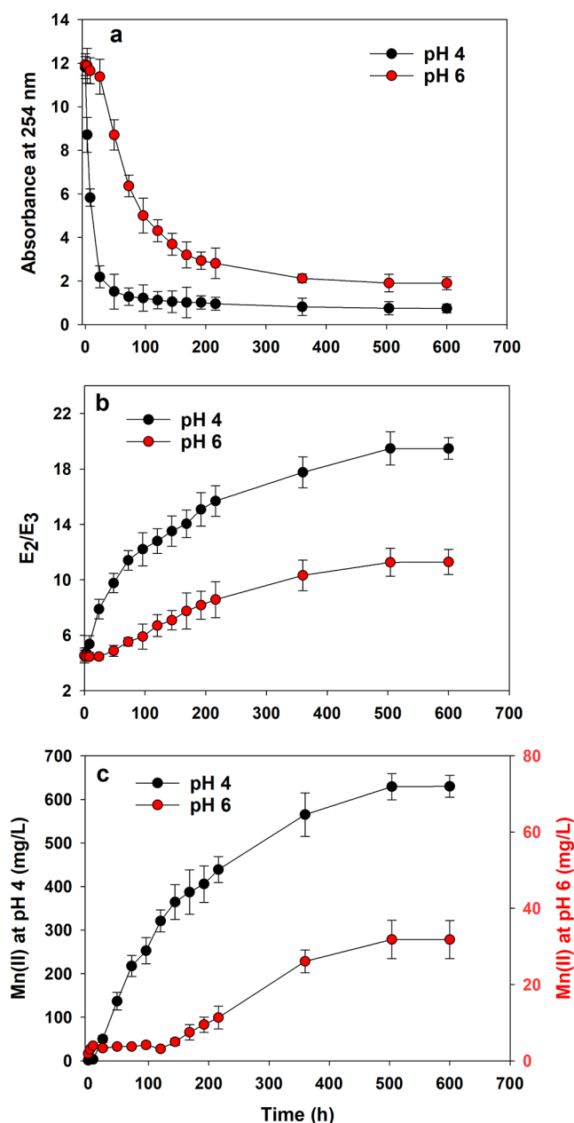
Figure 1. Ultraviolet absorbance at 254 nm (a), E_2/E_3 ratios (b), and Mn(II) concentrations (c) in the solution phase during the reaction of SRFA with \delta -MnO 2 at pH 4 and pH 6. The reported UV-vis absorbance values in (a) were the measured values multiplied by the dilution times. Details provided in Text S2.
