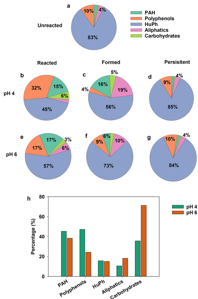
Figure 3. Abundance-weighted contributions of five compound classes to unreacted FA (a), and reacted (b, e), formed (c, f), and persistent compound pool (d, g) and percentage of the number of reacted compounds over the total number in each compound class (h). PAH, polycyclic aromatic hydrocarbons; Polyph, polyphenols; HuPh, highly unsaturated C and phenolic compounds; Aliph, aliphatic compounds; and Carbo, carbohydrates.
