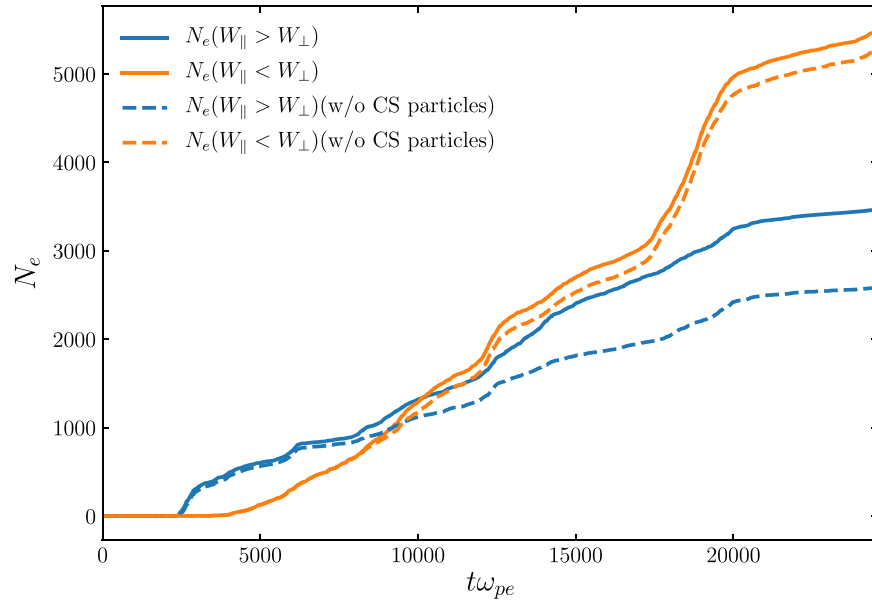
Figure A6. Number of particle dominated by W_{||} or W_{\perp} when crossing \gamma_{\text{inj}} = \sigma_e/2 in a larger box of 5440d_e \times 2720d_e . Compare with Figures 4 and A1.
