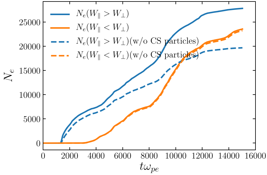
Figure B1. Number of particles crossing the lowered threshold \gamma_{\text{inj}} = \sigma_e/4 . Analogous to Figure 4.
