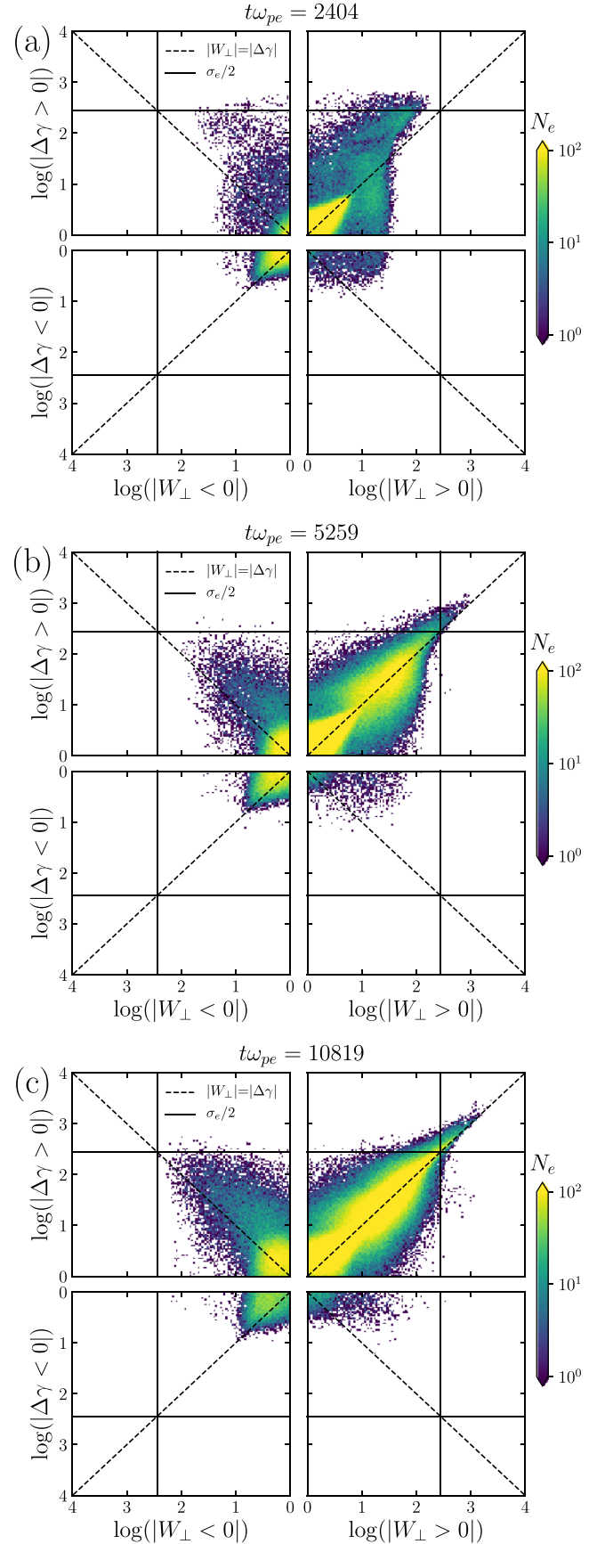
Figure 11. Contribution to energy gain/loss by the perpendicular electric field on all particles that started outside the current sheet.
