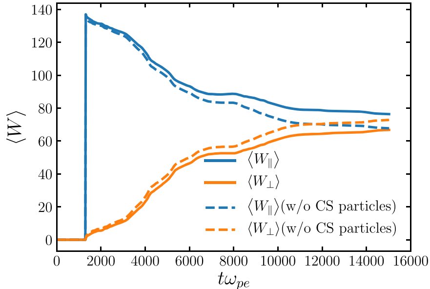
Figure B2. Average energy gain of particles crossing the lowered threshold \gamma_{\text{inj}} = \sigma_e/4 . Analogous to Figure 6(a).
