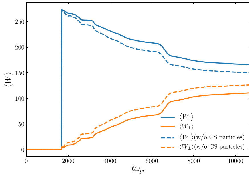
Figure A2. Average energy gain for particles crossing \gamma_{inj} = \sigma_e/2 in a smaller box of 1360d_e \times 680d_e . Analogous to Figure 6.
