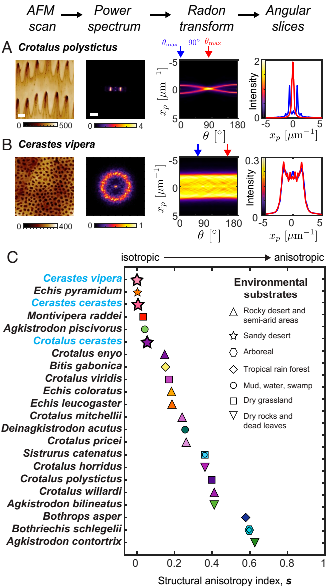
Fig. 4. Quantification of structural anisotropy. We define a structural anisotropy index, s , by taking the radon transform of the power spectrum and comparing the radial profiles of the radon transform along the dominant angular direction, \theta_{\max} , and the orthogonal direction, \theta_{\max} - 90^\circ . (A and B) These steps are shown for Cr. polystictus (A) and Ce. vipera (B). (C) The Jensen–Shannon divergence of the two radon profiles provides a quantification of the structural anisotropy (see Materials and Methods for details). The three sidewinding specialists investigated here (labeled with blue text) have nearly isotropic microtextures.
