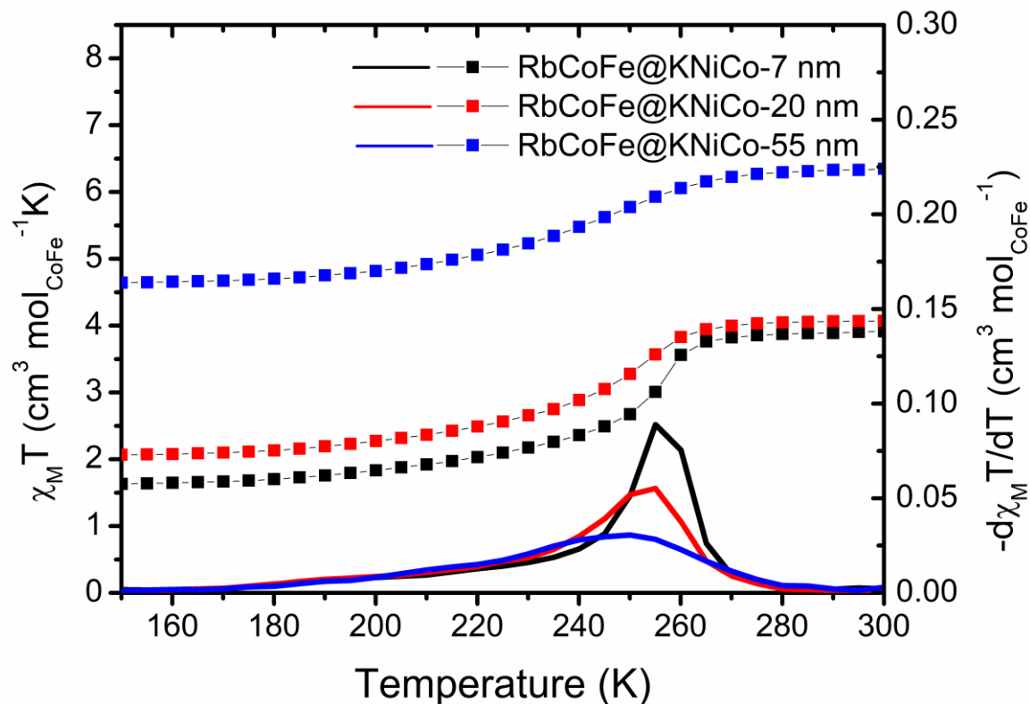
Fig. 2. \chi_M T vs T plots under a field of 100 G in the region of the thermal CTCST for the core-shell heterostructures. The derivatives of \chi_M T are plotted as solid lines.
