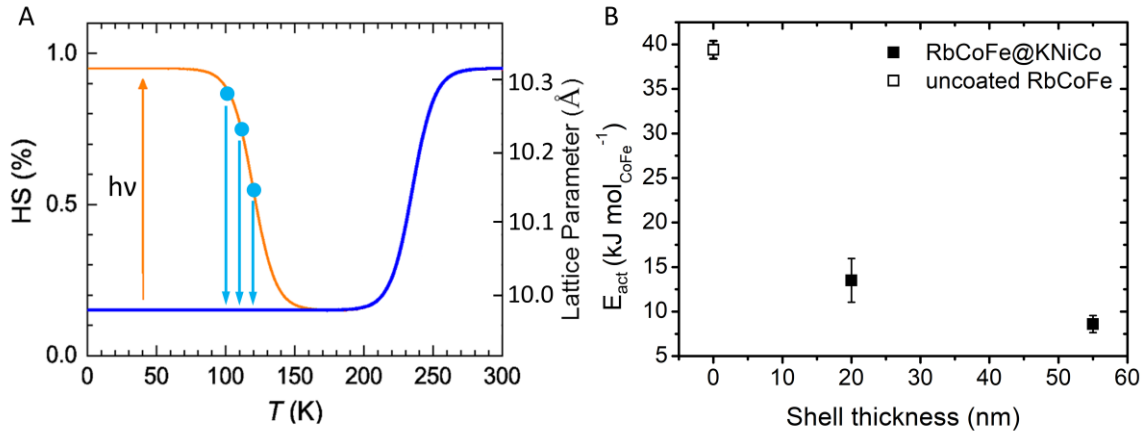
Fig. 4. (A) Schematic of the isothermal relaxation process. The sample is first cooled from room temperature (blue line) and the metastable HS state is established by light irradiation (yellow). The sample is then warmed to target temperatures (blue dots), where the decay of the HS state is monitored (blue arrows). (B) Activation energy vs shell thickness for the relaxation from the metastable HS state of RbCoFe-PBA as
