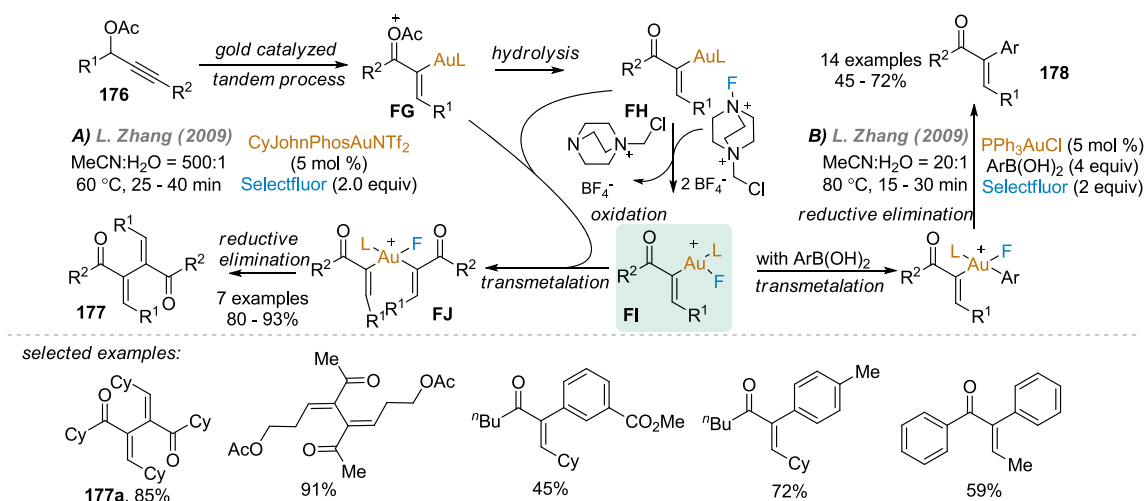
Scheme 83. Oxidative Homo- and Cross-Coupling of Propargylic Acetates
