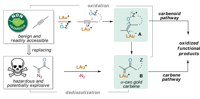
Scheme 1. Au-Catalyzed Oxidation of Alkynes by Nucleophilic Oxidants: General Reactivity and Comparison to Dediazotization
