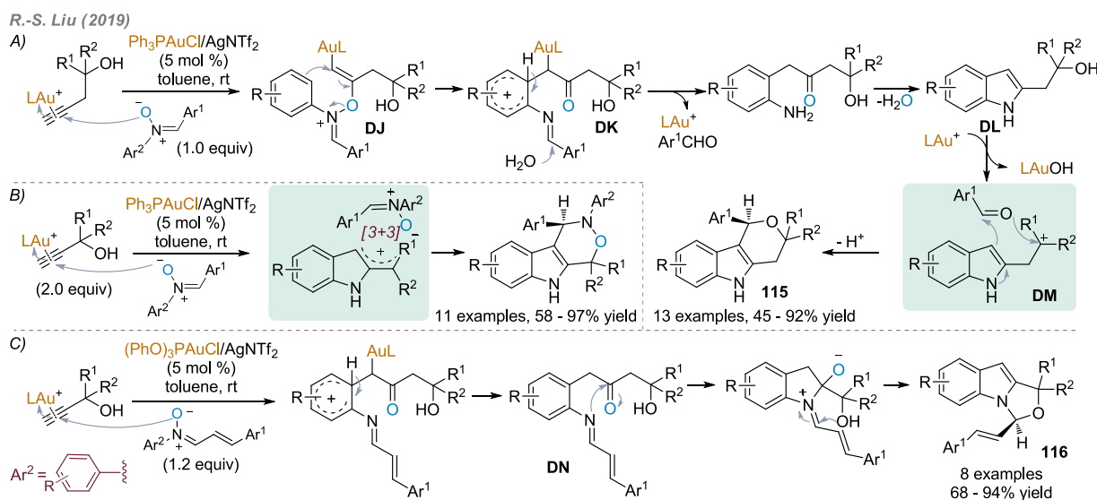
Scheme 61. Use of Nitron as an External Oxidant: Formation of Fused Indoles
