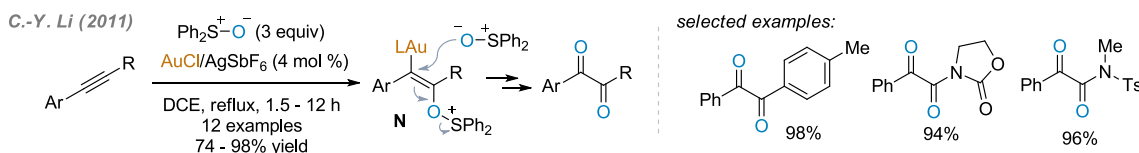
Scheme 7. Synthesis of 2-Acyl-1-naphthols via Gold-Catalyzed Oxidative Cyclization of 2-Alkenylphenyl Alkynyl Ketones
