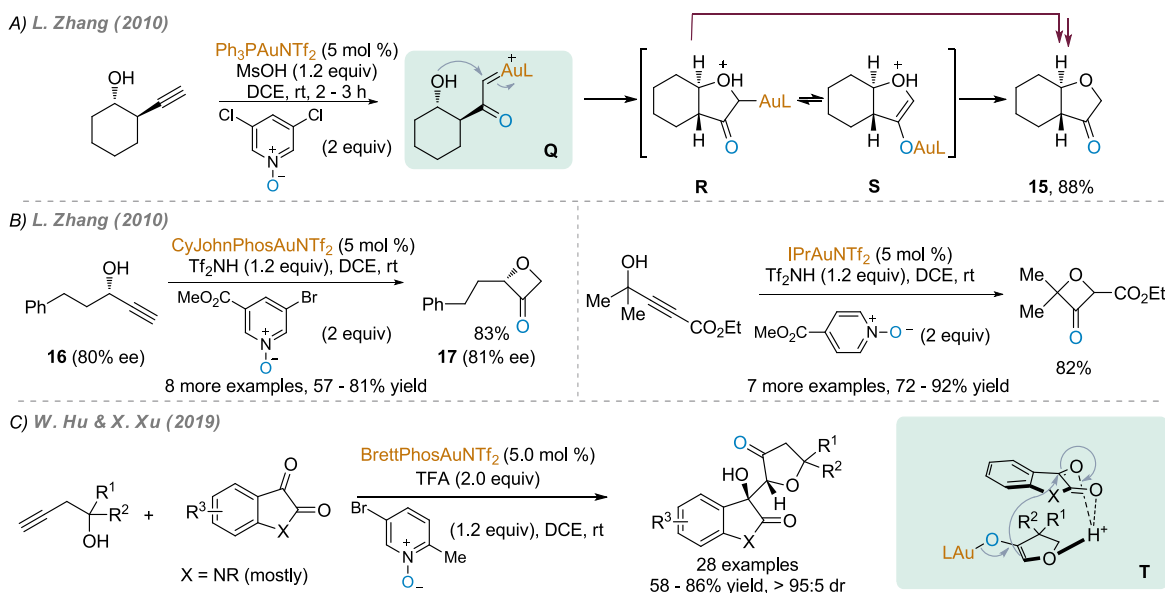
Figure 1. Commonly employed N -heteroarene N -oxides and their frequencies of occurrence in scope studies in reported oxidative gold catalyses (110 occurrences out of 102 papers).
