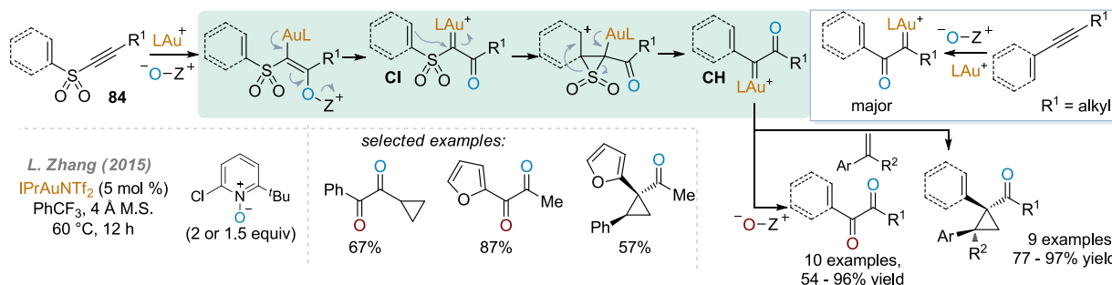
Scheme 47. Ring Expansion of Alkynyl Heterocycles through 1,2-Insertion into a Carbon–Heteroatom Bond by Gold Carbene
