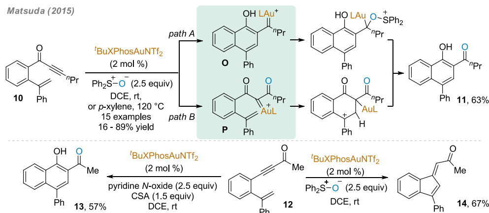
Scheme 7. Synthesis of 2-Acyl-1-naphthols via Gold-Catalyzed Oxidative Cyclization of 2-Alkenylphenyl Alkynyl Ketones
