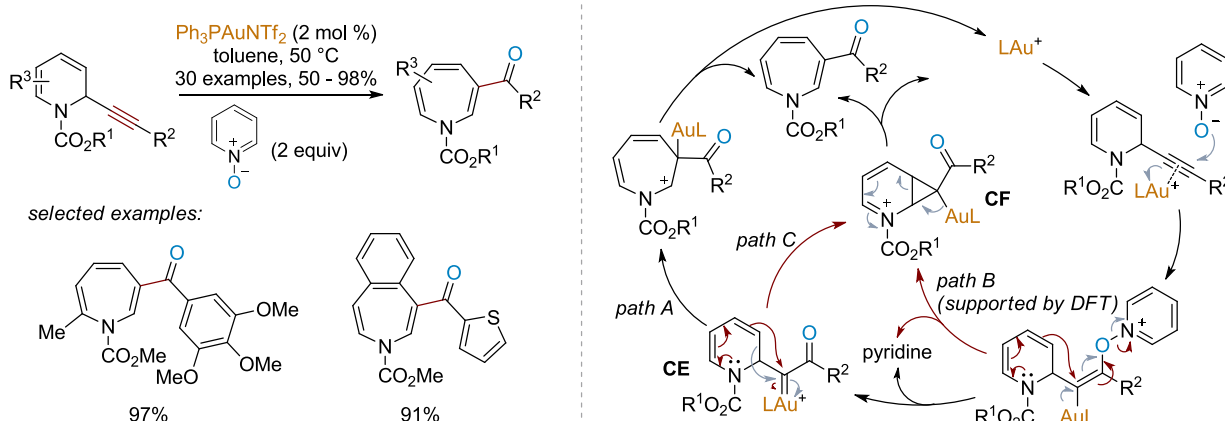
Scheme 45. 1,2-Enynyl/ o -Alkynylaryl Migration in Gold-Catalyzed Oxidation of Propargylic Silyl Ethers
