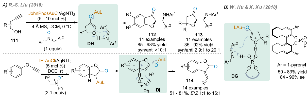
Scheme 61. Use of Nitron as an External Oxidant: Formation of Fused Indoles
