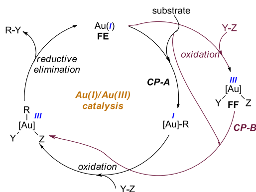
Scheme 82. Oxidative Au(I)/Au(III) Catalysis: Mechanistic Considerations
