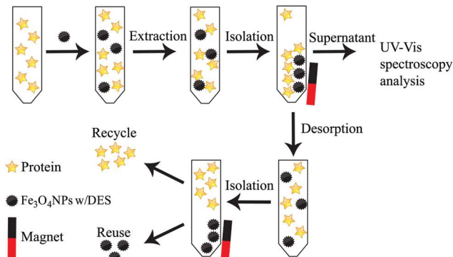
Fig. 5 General protein extraction process using magnetic iron oxide nanoparticles with deep eutectic solvents. Adapted with permission from ref. 44–46. Copyright © 2015, 2016 Elsevier.
