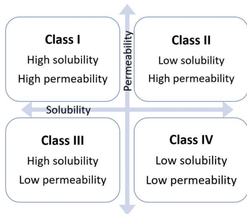
Fig. 12 Biopharmaceutical classification system of APIs reprinted with permission from ref. 163. Copyright © 2017 Elsevier.
