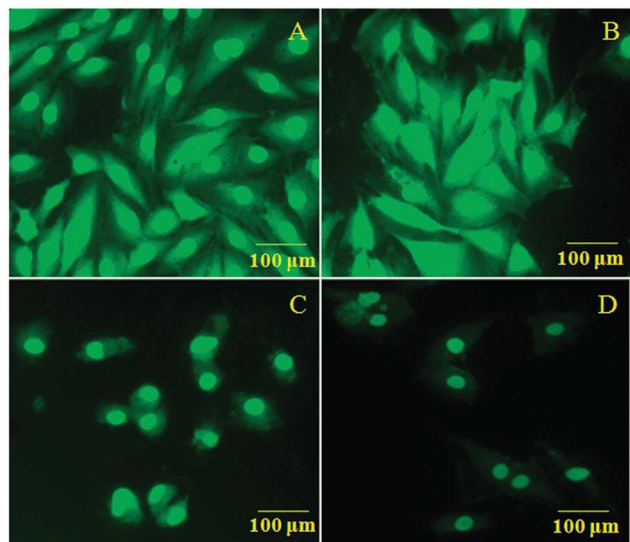
Fig. 13 Apoptosis of A549 cells cultured with CPT-loaded poly-cp-co-CA micelles for (A) 0 min, (B) 24 h, (C) 48 h and (D) 72 h. Reprinted with permission from ref. 172. Copyright © 2018 Royal Society of Chemistry.
