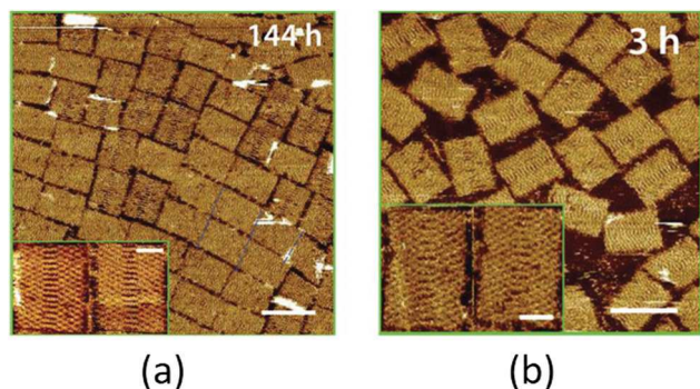
Fig. 6 AFM images illustrating the folding of DNA origami structures: (a) in anhydrous choline : glycerol (1 : 4) at 20 °C for 144 h; (b) in (hydrated) 75% choline : glycerol (1 : 4) at 20 °C for 3 h. Reprinted with permission from ref. 53. Copyright © 2015 Wiley.
