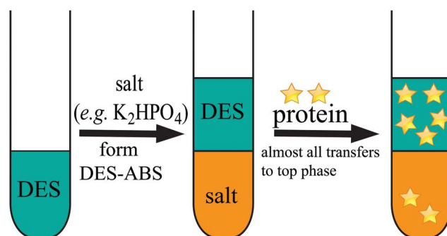
Fig. 4 General schematic of the extraction process of proteins using an aqueous biphasic system implementing deep eutectic solvents. Adapted with permission from ref. 37–39. Copyright © 2014 Royal Society of Chemistry; 2015, 2016 Elsevier.
