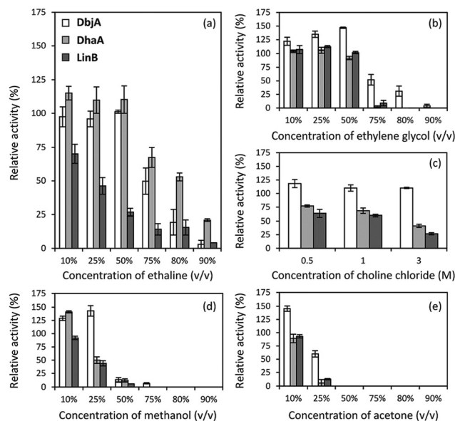
Fig. 10 The relative activities of DbjA, DhaA, and LinB measured in the presence of various concentrations of (a) ChCl:ethylene glycol (ethylene), (b) ethylene glycol, (c) choline chloride, (d) methanol, and (e) acetone at 37 °C and pH 8.6. Reprinted with permission from ref. 101. Copyright © 2014 Royal Society of Chemistry.
