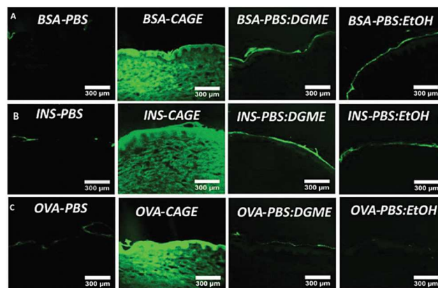
Fig. 14 Confocal images of skin penetration of fluorescently labeled proteins in PBS, CAGE, 50:50 (v/v) PBS:DGME, or 50:50 (v/v) PBS: ethanol. Reprinted with permission from ref. 203. Copyright © 2017 Wiley.
