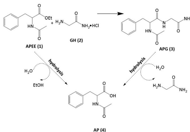
Fig. 9 Chymotrypsin-catalyzed reaction adapted with permission from ref. 99. Copyright © 2013 Wiley.
