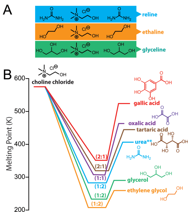
Fig. 1 (A) The “notorious three” DESs (i.e., reline, ethaline, glyceline) currently responsible for the bulk of the research activity in the area. (B) Diagram of select binary combinations of choline chloride with various hydrogen bond donor species illustrating the melting points of the constituents compared with the eutectic formed at the stoichiometry indicated. **It is noteworthy that the trend shown for 1:2 choline chloride:urea coincides nearly exactly with that of the 1:1 choline chloride:malonic acid system.
