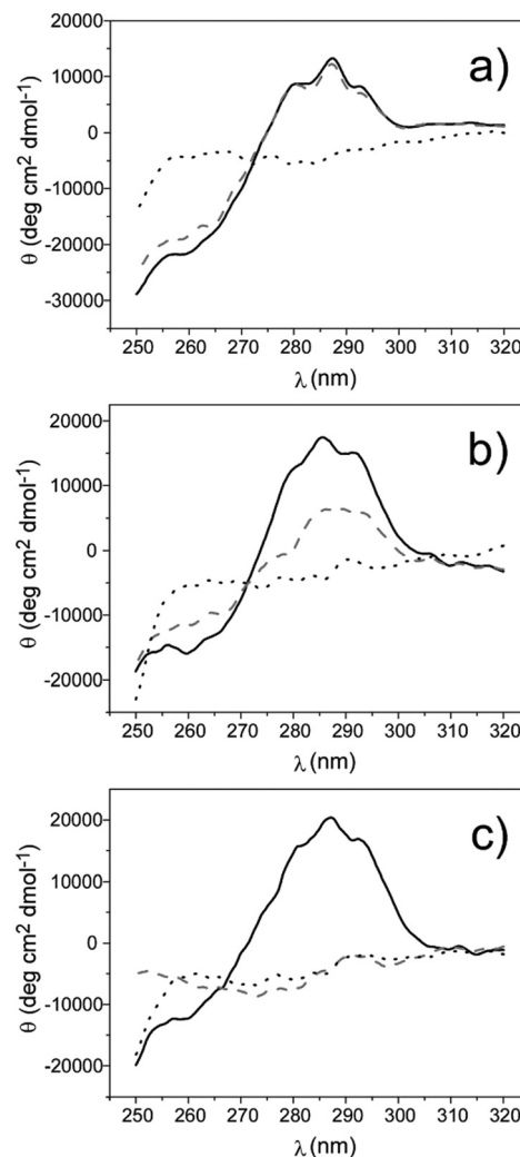
Fig. 2 Near UV CD spectra of lysozyme dissolved in MES buffer solution (a), neat ChCl:glycerol (b), and neat ChCl:urea (c), at 20 °C before thermal treatment (solid line), at 80 °C (dotted line), and at 20 °C after cooling (dashed grey line). Reprinted with permission from ref. 23. Copyright © 2012 Royal Society of Chemistry.
