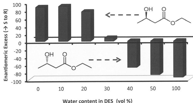
Fig. 11 Enantioselectivity of the reductive reaction depending on the different water/DES mixtures. Conditions include 50 mM ethyl acetoacetate and 200 mg mL -1 baker's yeast in 1:2 molar ratio of ChCl:glycerol at room temperature for 72 h. Reprinted with permission from ref. 109. Copyright © 2014 Wiley.
