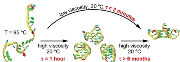
Fig. 7 DNA refolding in viscous choline chloride : urea (1 : 2 molar ratio). Reprinted with permission from ref. 60. Copyright © 2012 American Chemical Society.
