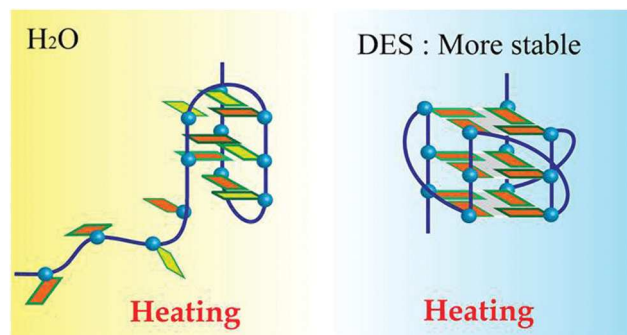
Fig. 8 Human telomeric DNA, Tel 22 , adopting a more stable parallel G-quadruplex structure in water-free DES (containing K + ). Reprinted with permission from ref. 61. Copyright © 2013 American Chemical Society.
