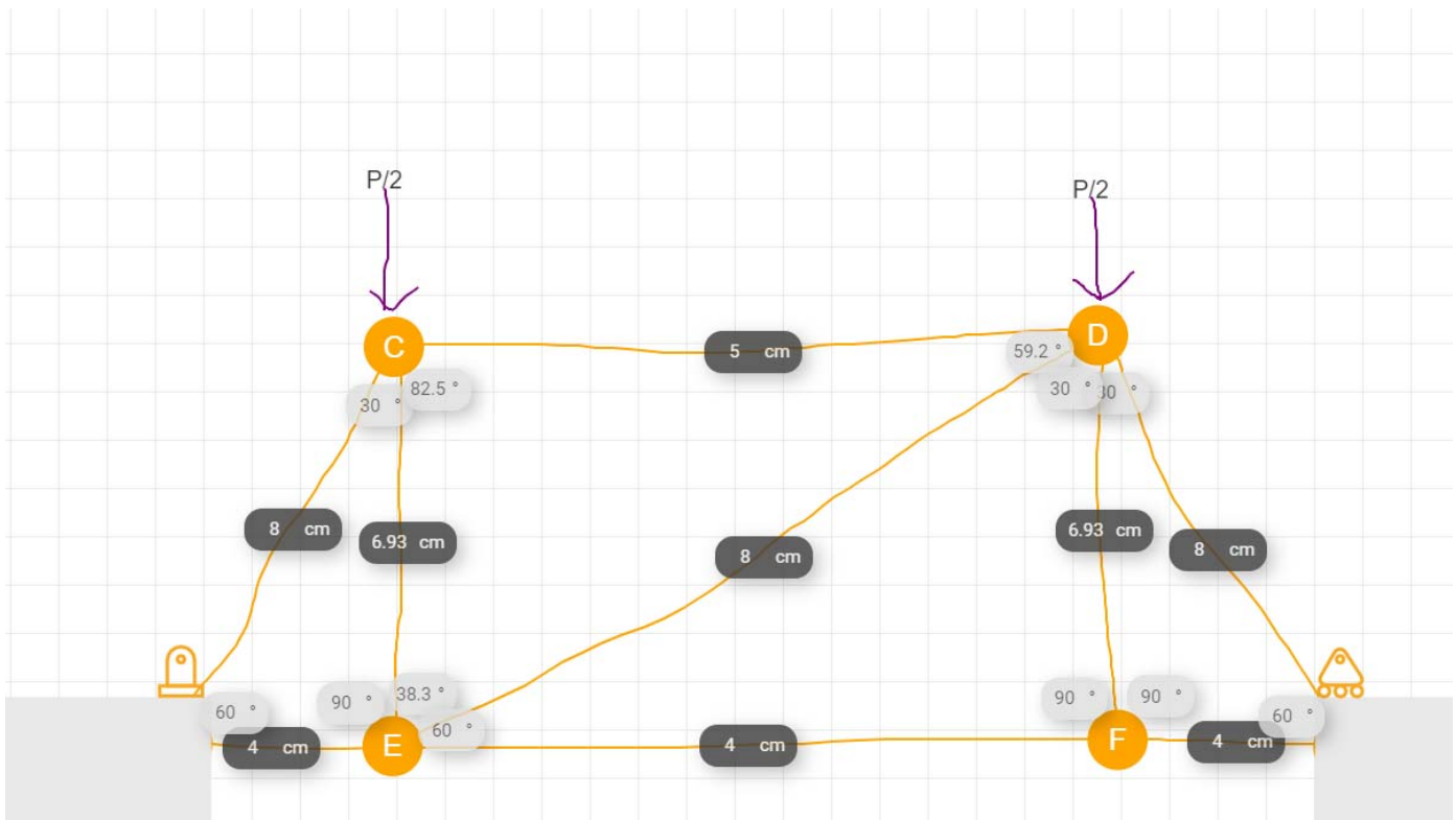
Figure 2: Example of Mechanics User Interface, with a drawn Truss system. This example comes directly from the Truss Design Mode, in which students are given freedom to develop their own solution to an open-ended question, in which they have to meet certain specifications set by the instructor while attempting to maximize the load that the truss can take.
