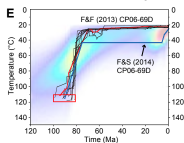
E. Westernmost Grand Canyon, ^4\text{He}/^3\text{He} Flowers & Farley (2013) versus Fox and Shuster (2014; colors), Separation Canyon.
