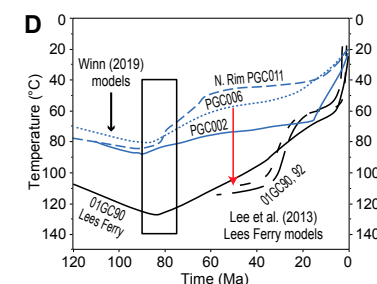
D. Marble Canyon (black) and Kaibab uplift (blue), Karlstrom et al. (2014); Winn (2019).
