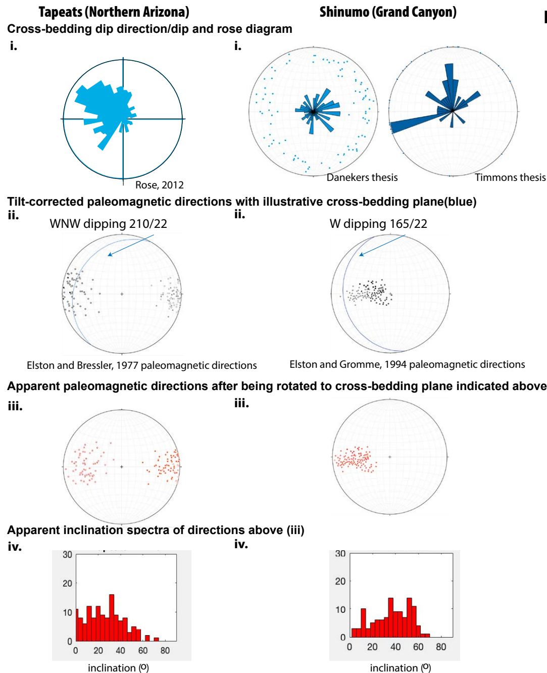
Figure 2 ( continued ). (E) Illustration of non-uniqueness of inclination data when cross-bedding versus bedding laminations cannot be distinguished. For both Tapeats (left) and Shinumo (right) sandstones of Grand Canyon, E.i. plots of paleoflow directions and dips (blue), E.ii. plots of the sample paleomagnetic directions (black) and an illustrative bedding plane (210/22 for Tapeats and 165/22 for Shinumo, both in blue), E.iii. plots of the apparent paleomagnetic directions, i.e., the measured paleomagnetic directions relative to horizontal (as plotted in E.ii) having been rotated about the strike of the indicated cross-bedding plane, resulting in the apparent paleomagnetic directions one might measure if bedding were confused with this orientation of cross bedding. E.iv. illustrates the overall inclination spectra of these apparent directions and shows the non-uniqueness of inclination data when cross bedding cannot be distinguished from bedding lamination.
