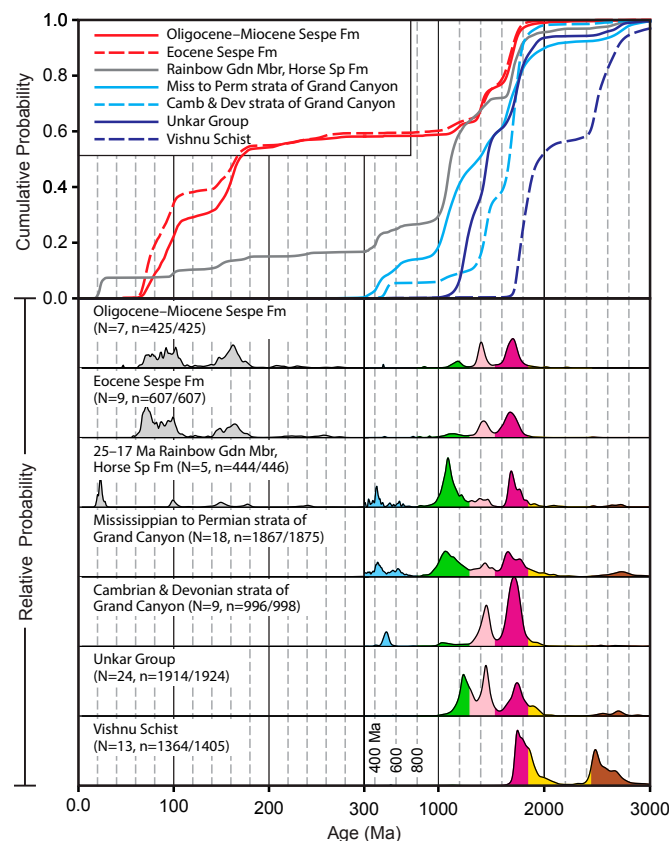
Figure 13. Illustration that if the Sespe Formation includes clasts derived from Shinumo Sandstone, then it should also include zircon populations found in the Proterozoic basement and Phanerozoic strata of Grand Canyon. This is not the case, as indicated by the scarcity of Archean, 2000–1800 Ma, 1100 Ma, latest Proterozoic (Gondwanan), and Paleozoic (Appalachian) zircon in both Eocene and Oligocene–Miocene parts of the Sespe Formation. Rather, the ages and proportions of pre-arc zircon in the Sespe Formation are typical of Cretaceous to Paleogene strata in southern California that are inferred to have been derived from sources in southern California, southwestern Arizona, and/or northwestern Sonora (Jacobson et al., 2011; Ingersoll, et al., 2013, 2018; Sharman et al., 2015). Similarly, the Rainbow Gardens Formation of the Grand Wash Trough, which lies along the course of the modern Colorado River, shows no obvious evidence of sediment contribution from the Devonian and older rocks exposed in the deeper parts of Grand Canyon. Note age-axis scale break at 300 Ma. For the probability density plot (PDP) panels, the vertical scales also differ to the left and right of the scale break, such that equal area represents equal probability throughout graph. “N” and “n” as in previous figures.
