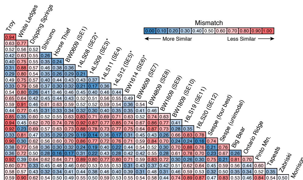
Figure 7. Dissimilarity matrix generated using Mismatch of probability density plots (PDPs) (Amidon et al., 2005) for individual Sespe clasts and subset composites compared to composite samples of Shinumo, Troy, Big Bear, Dripping Springs, White Ledges, Pinto Mountain, Horse Thief, Ontario Ridge, Pinto Mountain, Tapeats, and Zabriskie quartzites. All of the Sespe clasts are dissimilar to the Shinumo composite with Mismatch values ranging from 0.35 to 0.46 and also dissimilar to all of the individual Shinumo samples with Mismatch values ranging from 0.32 and 0.84 and with a mean of 0.55 \pm 0.15 ( 1\sigma ) (see the Supplemental Material [text footnote 1] for further quantitative comparison of individual samples and composite samples using each measure of dissimilarity. None of the four most Shinumo-like Sespe clasts (samples with asterisks) has a definitive or even moderately likely derivation from Shinumo Sandstone. See Table S3 for a full matrix that includes all individual clasts discussed herein.
