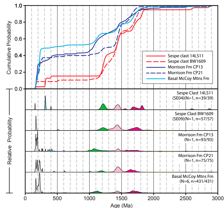
Figure 14. Sample 14LS11 has a maximum depositional age (MDA) of ca. 150 Ma, assuming the ages <500 Ma are not allochthonous. Sabbeth et al. (2019) concluded that this clast was derived from the Westwater Canyon Member of the Morrison Formation. Although not explicitly addressed by Sabbeth et al. (2019), we here also consider Sespe clast BW1609, which has a similar young apparent MDA. Both Sespe clasts have similar pre-arc age distributions as two samples of the Westwater Canyon member (CP13 and CP21) analyzed by Dickinson and Gehrels (2008a), but much lower proportions of arc-derived zircon, such that a correlation between the Sespe clasts and Morrison Formation is not compelling. Quartz arenite of Late Jurassic to Early Cretaceous age is exposed in several areas in southern California and southwestern Arizona. One example is the McCoy Mountains Formation (Barth et al., 2004; Spencer et al., 2011), but as with the Morrison Formation, the abundance of arc-derived zircon is much higher than in the Sespe clasts. Note that the above comparisons are constrained by only 39 and 57 dated zircon grains, respectively, from the two Sespe clasts.
