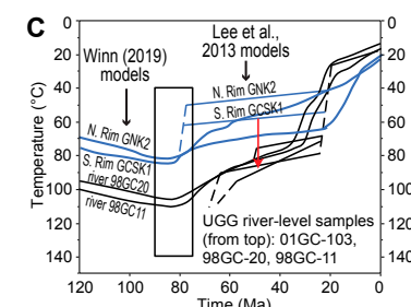
C. Eastern Grand Canyon AHe and AFT, Lee et al. (2013), Winn (2019).
