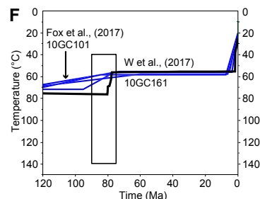
F. Westernmost Grand Canyon, combined ^4\text{He}/^3\text{He} , AFT, and AHe, (Winn et al., 2017) and ^4\text{He}/^3\text{He} (Fox et al., 2017, blue), Separation Canyon.
