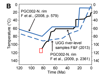
B. Eastern Grand Canyon, AHe and ^4\text{He}/^3\text{He} , Flowers and Farley (2013). Blue = rim samples.
