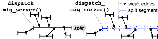
Figure 5: The segment for batch processing in dispatch_mig_server is split into multiple segments to distinguish different items. Weak edges are added among the split segments.
