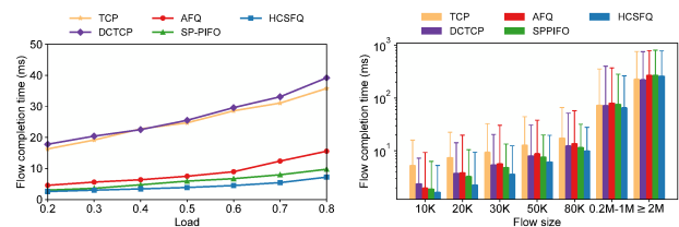
(a) Average flow completion time for flows less than 100KB.
