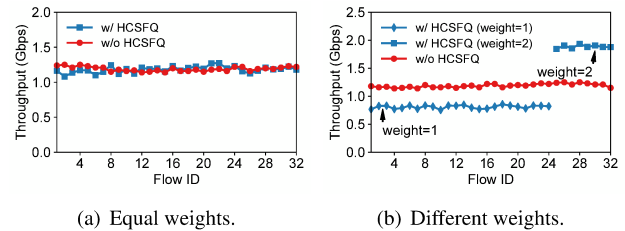
Figure 8: Testbed experiments of fair queueing for TCP.
