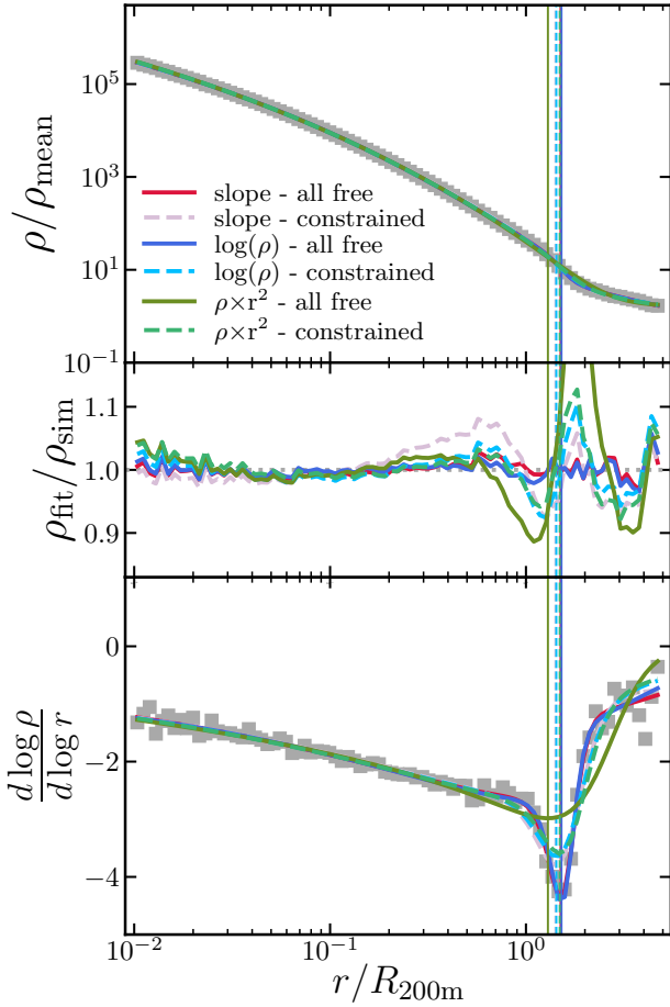
Figure 2. The stacked density profile from TNG300-1-DM for haloes with 10^{14.5} M_{\odot} < M_{200m} < 10^{15} M_{\odot} at z = 0 . We test six fitting methods using Equation 6 or 10. The red lines fit the logarithmic slope directly using Equation 10, the blue lines fit the profile using the log of Equation 6 and the green lines fit the profile using Equation 6 multiplied by r^2 . The darker solid lines leave all eight parameters in the fitting function free, while the lighter dashed lines constrain three parameters according to empirical trends and use five free parameters. The vertical lines show R_{sp} for each fitting method found by identifying the minimum of the analytic derivative. Each fit follows the sharp decline in the slope to a varying degree, and there is a small difference in the resulting value for the splashback radius.
