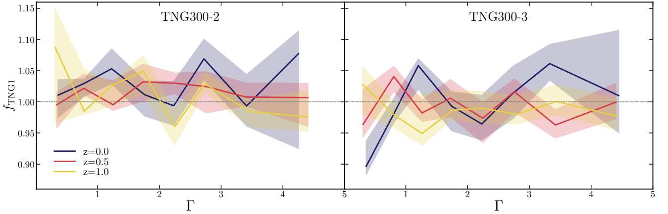
Figure A2. We show the fractional difference between R_{sp} in TNG300-1 and TNG300-2 (left) or TNG300-3 (right) calculated as a function of accretion rate \Gamma . The colours show several redshifts. Each resolution level has (\frac{1}{2})^3 as many particles as the previous resolution level. The haloes are stacked based on accretion rates in eight bins between 0 and 5. We compute the splashback radius of the median profile for each accretion range as described in Section 3.2.3.
