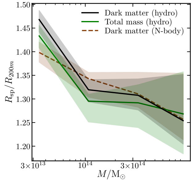
Figure 11. Location of the splashback radius as a function of halo mass for the dark matter and total mass in a hydrodynamic simulation (solid lines) and the dark matter mass in an N -body simulation (dashed line) at z = 0 . We stack the density profiles for haloes with \log_{10}(M_{200\text{m}}/M_{\odot}) in 13–13.5, 13.5–14, 14–14.5 and 14.5–15 and compute the splashback radius of the median profile, shown by the solid and dashed lines. To estimate error, we use a bootstrap method and show the 16th and 84th percentiles as the shaded band around each line. We do not find a significant difference between the hydrodynamic and N -body simulations for R_{\text{sp}}/R_{200\text{m}} as a function of halo mass.
