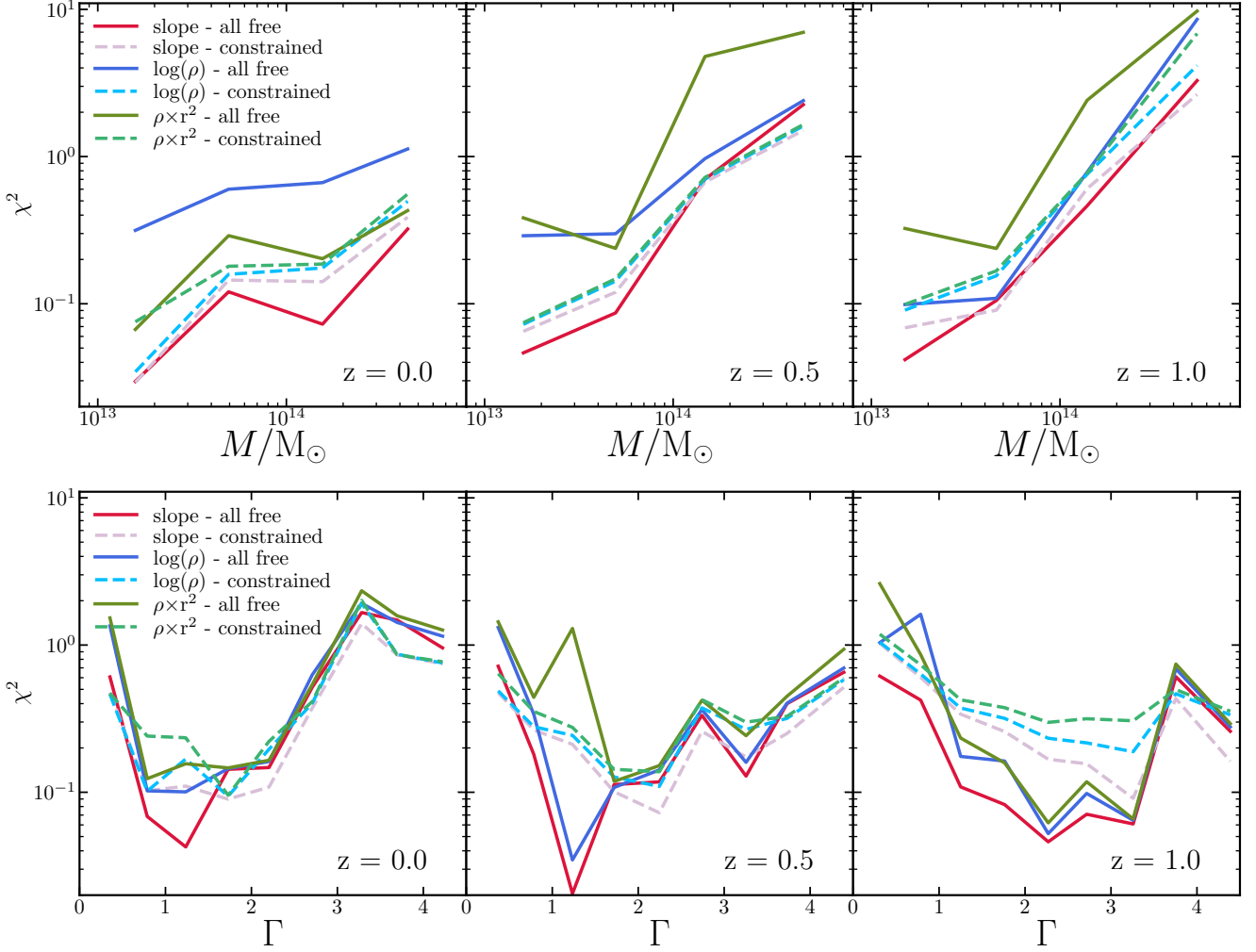
Figure 3. The \chi^2 value defined as in Equation 14 as a function of halo mass (top) or accretion rate (bottom) for redshifts 0, 0.5 and 1 (left, middle, and right panels). The difference between the numerical logarithmic derivative and the analytic logarithmic derivative is computed for points between 0.8R_{200m} and 2R_{200m} , which encloses the splashback region for all our profiles. The red lines show \chi^2 obtained from minimising the fit to the slope, the blue lines are obtained from minimising \log(\rho) and the green lines are obtained from minimising \rho \times r^2 . Solid lines leave all parameters from Equation 6 free, and dashed lines fix \alpha , \beta , and \gamma . The solid red line, fitting the slope with all parameters free, produces consistent fits across haloes and redshifts and is the method we use for the remainder of our results.
