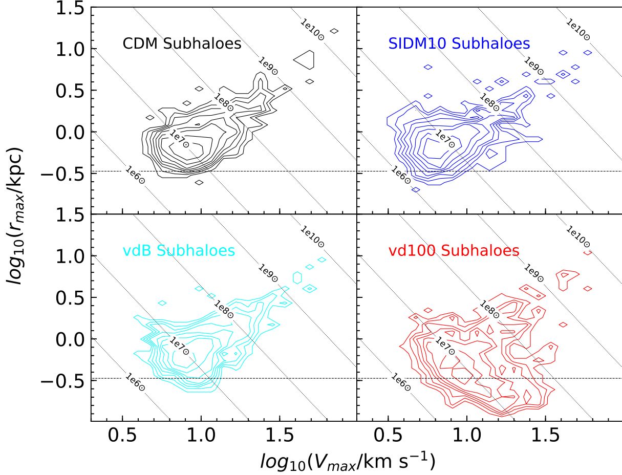
Figure 7. The V_{\max} - r_{\max} parameters for the CDM, SIDM10, vdB and vd100 subhalo samples, shown in the top left, top right, bottom left and bottom right panels respectively. The horizontal dashed line in each panel represents the 2.8 \epsilon softening resolution limit. the dotted lines indicate the V_{\max} - r_{\max} combinations that correspond to a fixed mass contained within r_{\max} as indicated in each panel.
