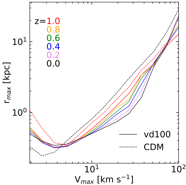
Figure 10. The evolution of the simulated vd100 dark matter subhalo V_{\max} - r_{\max} parameters over time. The circular velocity profile for the same subhaloes modelled under the CDM regime can also be seen at redshift values of z = 1 and z = 0 for comparison, plotted as dashed lines. The colours plotted correspond to a redshift of z = 1 (red), z = 0.8 (yellow), z = 0.6 (green), z = 0.4 (blue), z = 0.2 (violet) and z = 0 (black).
