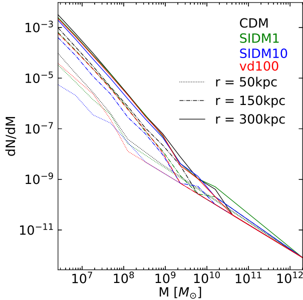
Figure 5. Differential subhalo mass function for all dark matter models considered, binned by radii from the centre of the host halo. Our three radial bins, < 50 kpc, < 150 kpc and < 300 kpc are denoted by dotted, dot-dashed and solid lines, respectively. The SIDM1, SIDM10 and vd100 models are denoted as green, blue and red solid lines respectively. The CDM model is denoted by black lines.
