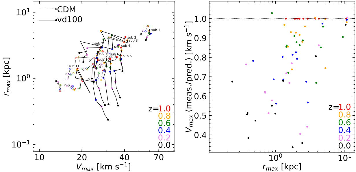
Figure 11. Left-hand panel: The evolution of the V_{\text{max}}-r_{\text{max}} parameters from z = 1 to z = 0 for 11 vd100 and 11 CDM subhaloes. The coloured dots represent the V_{\text{max}}-r_{\text{max}} parameter for the subhalo at the given redshift, the black lines trace the evolutionary track for the individual halo, moving from red ( z = 1 ) to black ( z = 0 ). The CDM data are shown with empty circles and dotted lines, and vd100 with filled circles as solid lines. Right-hand panel: the ratio of V_{\text{max}} (measured) to V_{\text{max}} (predicted) for the vd100 model, shown as a function of the corresponding r_{\text{max}} for 11 individual subhaloes from z = 1 to z = 0 .
