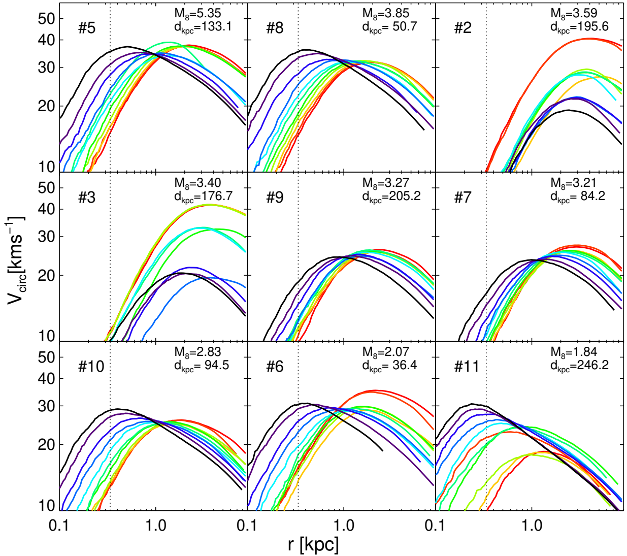
Figure 13. Same as Fig. 12 but for the circular velocity profiles.
