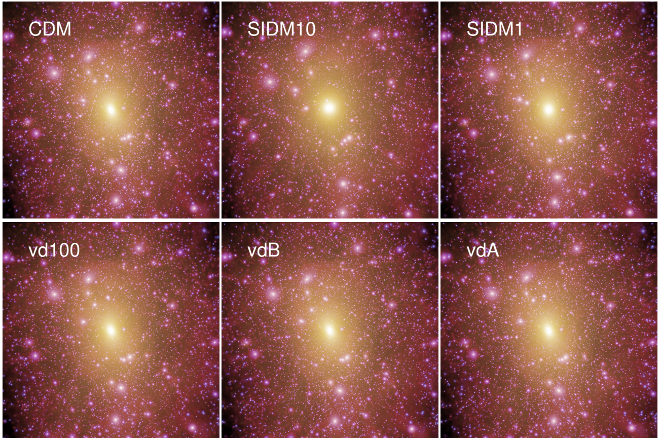
Figure 2. Images of the six haloes used in this study. The image intensity correlates with the dark matter column density and the the colour traces the velocity dispersion. Each image is 400 kpc on a side. The six simulations, from left to right and top to bottom, are: CDM, SIDM10, SIDM1, vd100, vdB and vdA.
