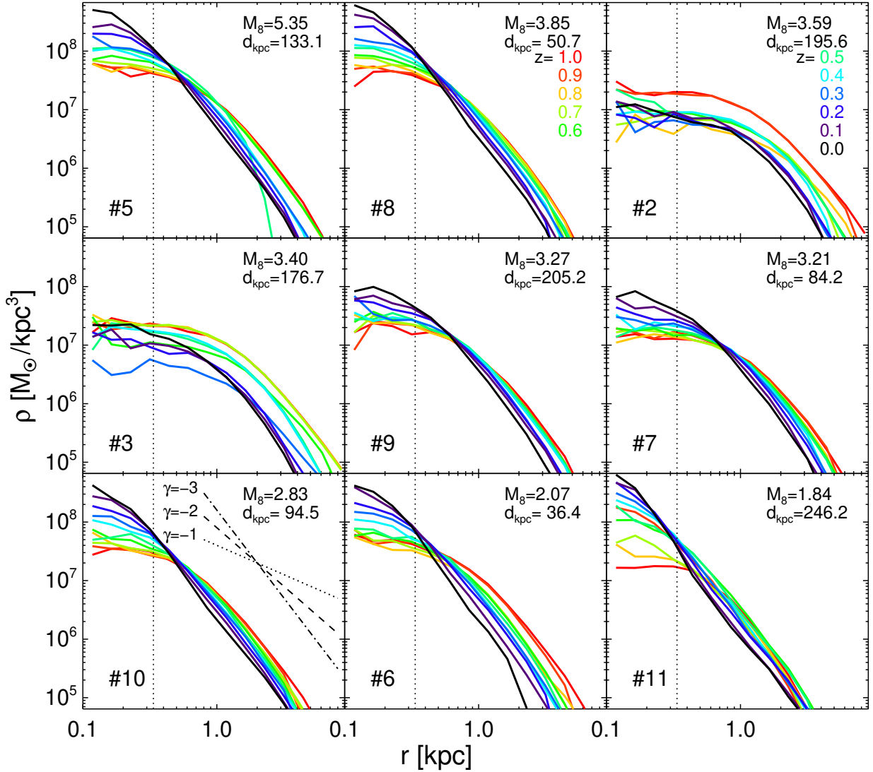
Figure 12. Density profiles for nine of the 11 haloes presented in Fig. 11, with the correspondence indicated by the number in the bottom left hand corner of each panel; we also include the z = 0 subhalo mass in units of 10^8 M_\odot and the z = 0 distance from the main halo centre. We show density profiles at 11 redshifts, which are shown with different colours evolving from red at z = 1 to black at z = 0 . The dotted vertical lines indicate the radius equal to 2.8 times the softening length, and therefore mark the hard resolution limit of our simulations. In the bottom left-hand panel we indicate power law slopes with indices -1, -2, and -3 as dotted, dashed, and dot-dashed lines respectively.
