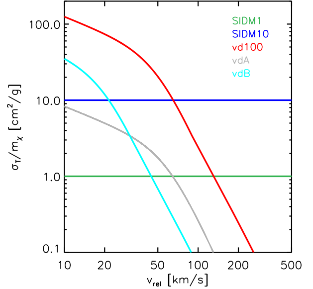
Figure 1. Cross-sections of the SIDM models used in this paper, presented as a function of relative velocity. These models are: SIDM1 (green), SIDM10 (blue), vd100 (red), vdA (grey) and vdB (cyan).
