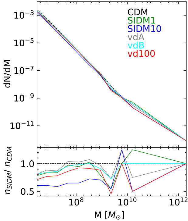
Figure 4. Differential subhalo abundance as a function of enclosed mass for all dark matter models considered. The SIDM1, SIDM10, vd100, vdA and vdB models are denoted as green, blue, red, grey and cyan solid lines respectively. The CDM model is denoted by a black dashed line. The bottom panel shows the mass function of all SIDM models as a ratio to that of the CDM model.
