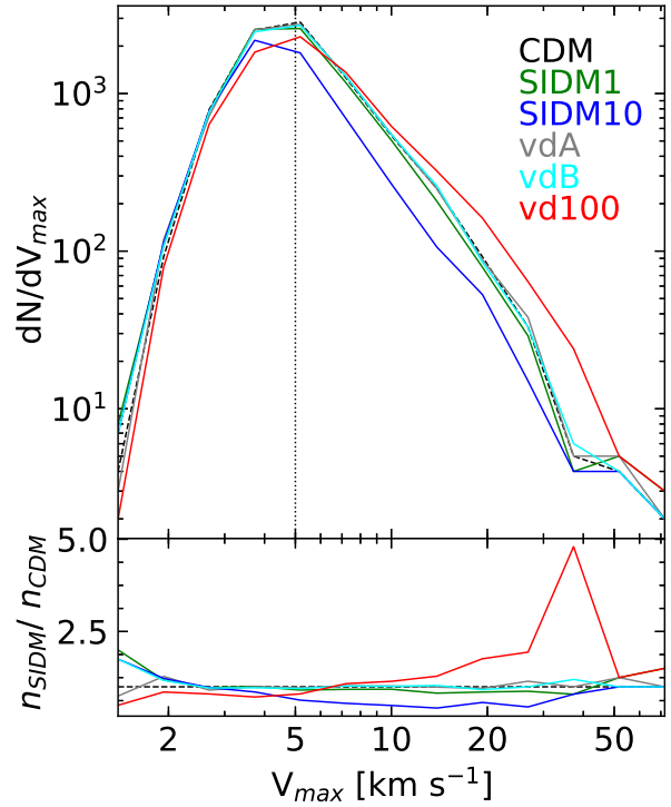
Figure 6. Differential subhalo V_{\max} function for all SIDM models considered, plus the CDM model. The SIDM1, SIDM10, vd100, vdA and vdB models are denoted as green, blue, red, grey and cyan solid lines respectively. The CDM model is denoted by a black dashed line. The dotted vertical line shows the resolution limit of the simulations. The bottom panel shows the V_{\max} function of all SIDM models as a ratio to that of the CDM model.
