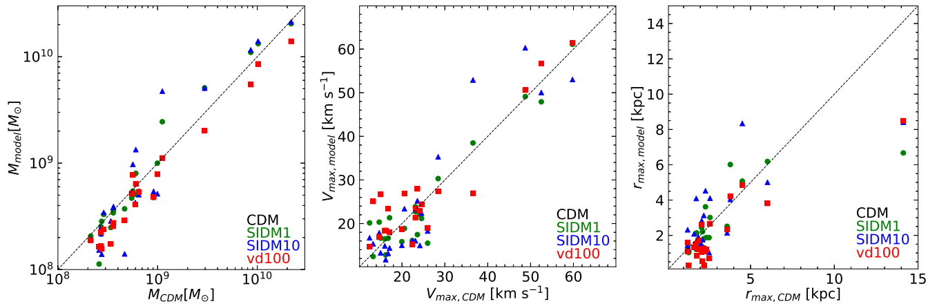
Figure 8. The properties of the same 22 subhaloes in the SIDM and CDM models matched between runs. In all three plots the vd100 model is denoted by red squares, the SIDM10 model by blue triangles and the SIDM1 model by green circles. Left: the bound mass of 22 matched subhaloes as simulated by the vd100 model and the SIDM models SIDM1 and SIDM10 shown in respect to the CDM model. Middle and right: the relationships between the aforementioned SIDM models and the CDM model in terms of V_{\max} and r_{\max} respectively.
