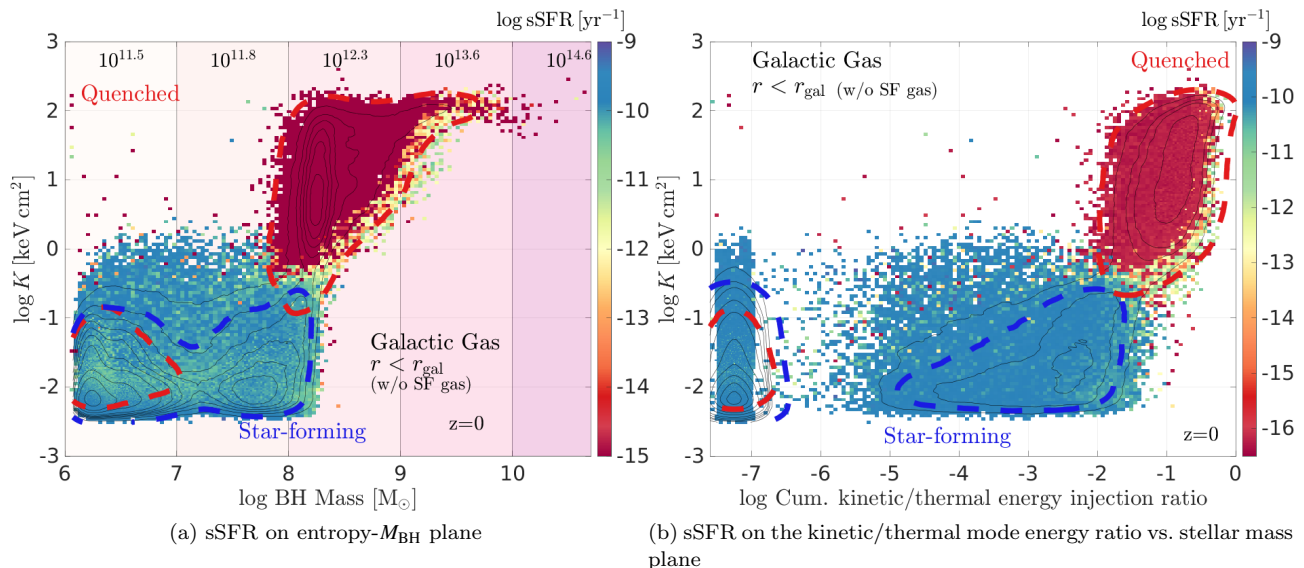
Figure 5. The role of the AGN feedback in setting the entropy and SFR of the galaxy. The distribution of z=0 TNG300 galaxies in the entropy- M_{BH} plane, with sSFR shown by colour (a), shows that the jump in galactic gas entropy and SF quenching occur at a sharp BH mass scale, where the energy injection of kinetic mode feedback becomes comparable to the thermal mode. This can be seen in (b) where the entropy is shown vs. the ratio between the cumulative energy injected by the two accretion modes, coloured by sSFR as before. The vertical band of points on the left of the plot are galaxies which have not experienced a single kinetic mode injection event, and are given a random value < 10^{-7} for the ratio. Red and blue contours enclose 90 per cent of the SF/Quenched populations respectively. The onset of quenching occurs when the kinetic mode energy becomes appreciable ( > 1\% of the thermal mode).
