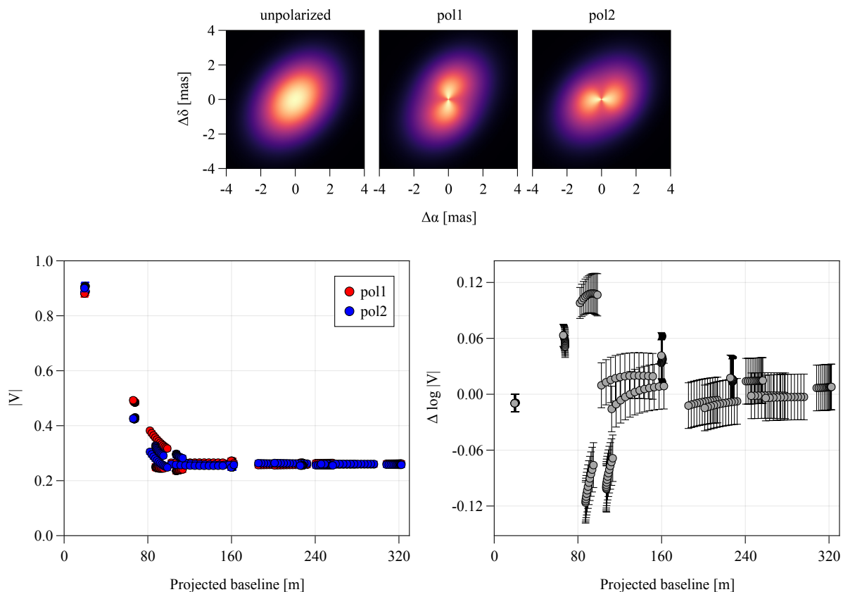
Figure 1. A simulated MIRC-X polarimetric observation of YSO star HD 163296 at 1.6\ \mu\text{m} , assuming a toy model Gaussian circumstellar disk with 20 % radial linear polarization. Top: “Images” of the modeled disk 14 in unpolarized and polarized emission. Bottom left: Modeled polarized visibility amplitudes for 6 telescope observations based on typical CHARA u-v coverage for this star. Bottom right: Differential polarized visibility amplitude (pol1/pol2 plotted in log scale) for the same synthetic measurements, with conservative error estimates (higher SNR is expected after proper calibration). Our simulations of various disk models indicate that a clear signal should be observable at intermediate baselines.
