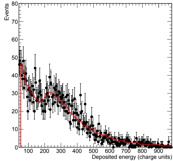
Fig. 16 Measured energy distribution for a single ECal crystal, in charge units, for cosmic-rays events selected according to the algorithm described in the text. The red curve represents the result of the fit performed using the template shape obtained from Monte Carlo simulations. (Color online).
