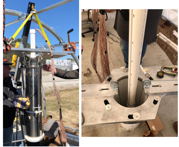
Fig. 2 Some pictures of BDX-Mini detector positioning phases. Left Panel shows the BDX-mini detector inside the stainless-steel watertight cylindrical vessel. Right Panel shows the detector lowering phase in the pipe: a PVC segment with the attached tape is clearly visible.
