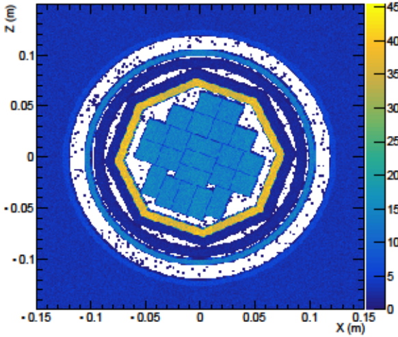
Fig. 10 Distribution of neutrino interaction vertices (in arbitrary units) in the BDX-MINI detector as obtained from the GENIE simulation. The color scale reflects the interaction probability and therefore the density of detector materials. Cyan: \text{PbWO}_4 crystals, yellow: tungsten shielding, dark blue: IV and OV, light blue: stainless steel vessel, white: air between vessel and PCV pipe, blue: PCV pipe and surrounding dirt. (Color online).
