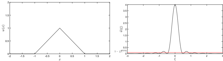
Fig. 1 Left panel, triangular filter (16) with L = 1 . Right panel, in black the Fourier transform (17) and in red the threshold value 1 - \sqrt{\gamma}
