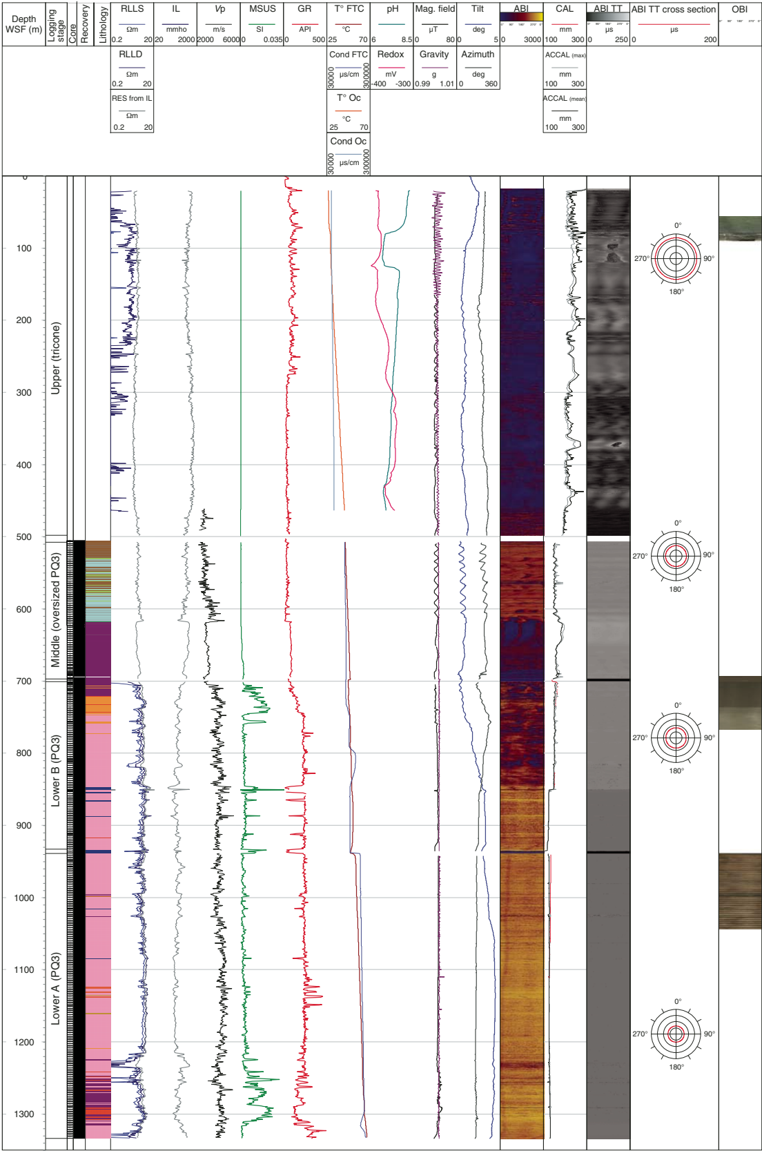
Figure F13. Wireline downhole log data, Hole M0077A. Shallow and deep reading resistivity (RLLS and RLLD), resistivity from induction (Res from IL), conductivity (IL), P-wave sonic ( V_p ), magnetic susceptibility (MSUS), total gamma ray (GR), borehole fluid temperature ( ^{\circ}\text{T TFC} ), conductivity (Cond FTC), pH and redox, gravity and local magnetic field, borehole tilt and azimuth, amplitude and traveltime acoustic images (ABI Amplitude and ABI TT), borehole diameter (CAL and ACCAL), traveltime cross section of the borehole (ABI TT cross section) and optical borehole image (OBI) See Figure F12 for lithology key.
