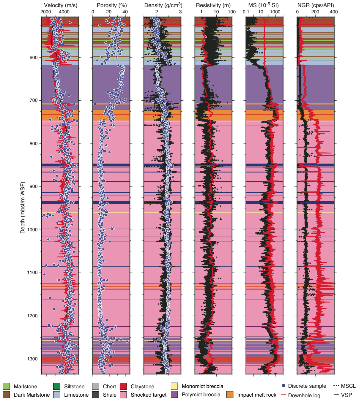
Figure F12. Physical property data, Hole M00077A.
