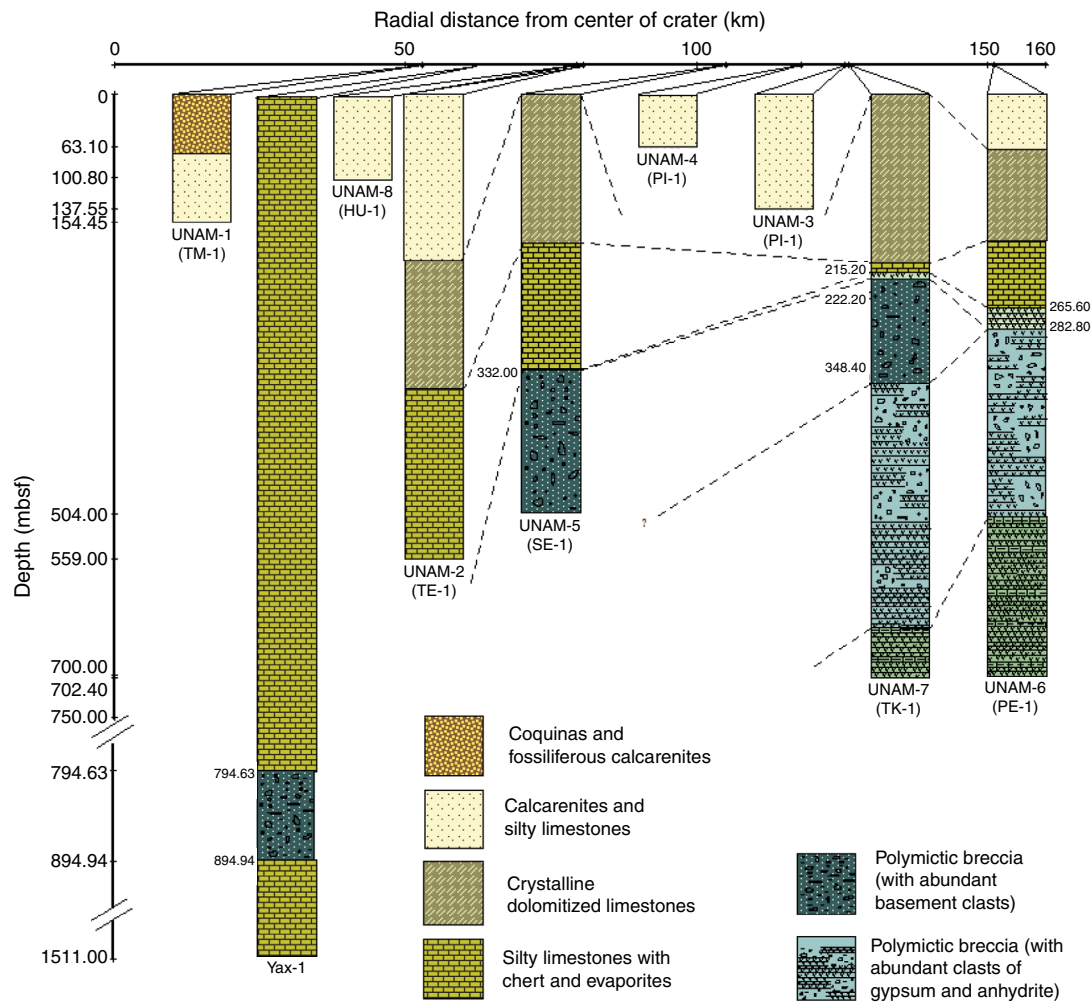
Figure F6 (continued). C. Lithologic columns and stratigraphy from UNAM and Yax-1 boreholes.
