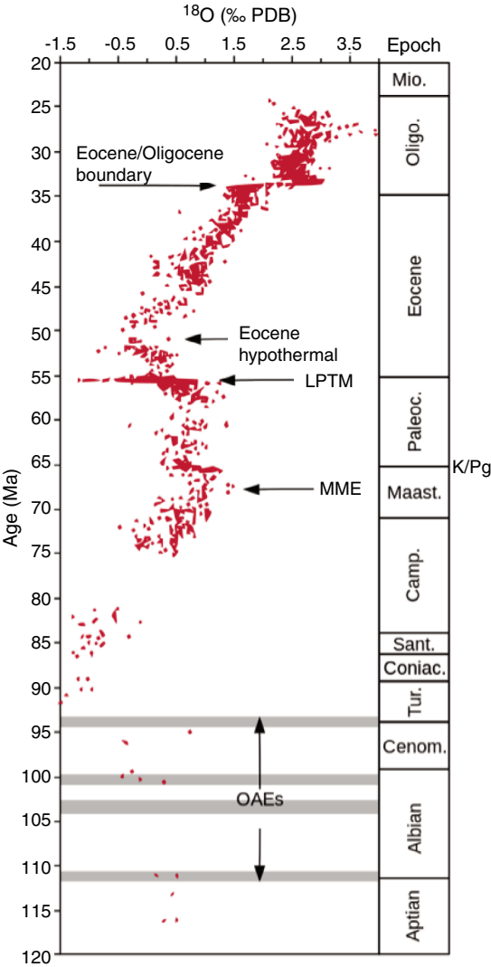
Figure F9. Generalized climate curve for the Cretaceous and Paleogene derived from deep-sea benthic oxygen isotope data (Zachos et al., 1993, 2001). Also shown: Eocene/Oligocene boundary, PETM, late Paleocene biotic event (LPTM), Cretaceous/Paleogene (K-Pg) boundary, mid-Maastrichtian event (MME), and early Aptian Oceanic Anoxic Event (OAE1a). Modified from the Leg 198 Synthesis (Bralower et al., 2006).
