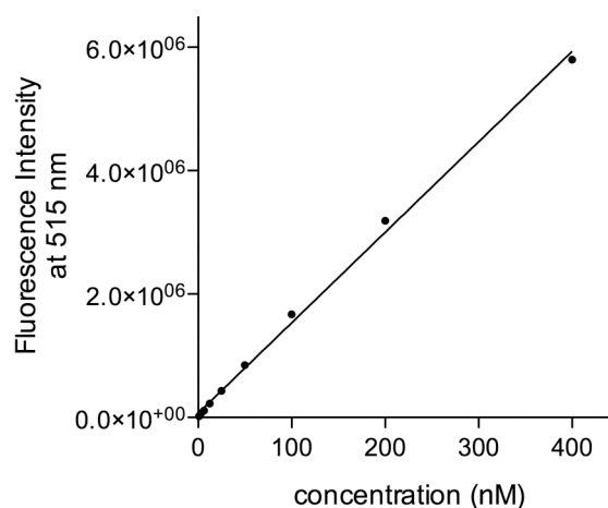
Figure S4. The relationship between fluorescence intensity and the concentration of compound 13 . The fluorescence intensities of compound 13 in 1% DMSO/50 mM phosphate pH 8 buffer were measured at various concentrations (0.78, 1.56, 3.13, 6.25, 12.5, 25, 50, 100, 200, and 400 nM) of 13 . Fluorescence Intensity = 14670•[ 13 ] + 66368. R^2 = 0.9974 . The equation was calculated using Microsoft Excel.
