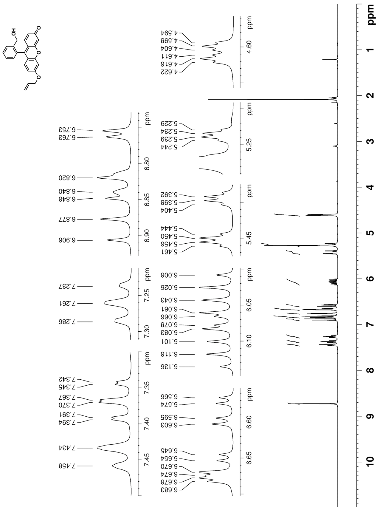
Figure S12. 1 H NMR spectrum of compound 11 (300 MHz, acetone-d 6 , 293K)
