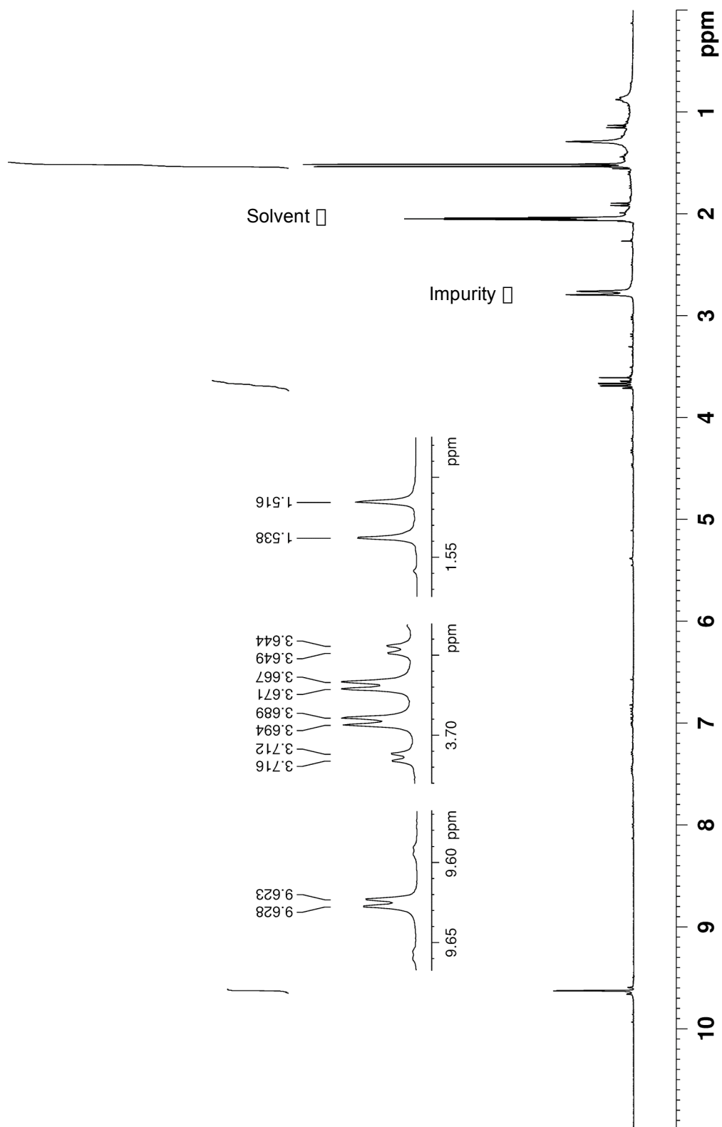
Figure S9. ^1\text{H} NMR spectrum of compound 8 (300 MHz, acetone- d_6 , 293K)
