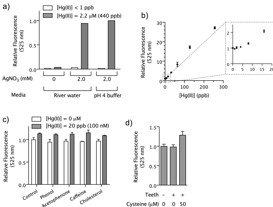
Figure 3. Applications of probe 3 for the detection of mercury species in environmental and dental samples. All detection was performed after adjustment of pH of samples to pH 4. (a) Comparison of river water and commercial pH 4 buffer ( [\text{HgCl}_2] = 2.2 \mu\text{M} (440 ppb)). In the absence of \text{AgNO}_3 , \text{Hg(II)} cannot be detected by the method (left). In the presence of \text{AgNO}_3 , \text{Hg(II)} can be detected (middle). (b) Mercury detection in river water ( [\text{HgCl}_2] = 0\text{--}256 ppb, [\text{AgNO}_3] = 2.0 mM). (c) Mercury detection in river water in the presence of organic compound ( [\text{AgNO}_3] = 2.0 mM, [\text{compound}] = 100 ppb). (d) Dental samples ( [\text{NCS}] = 500 \mu\text{M} ).
