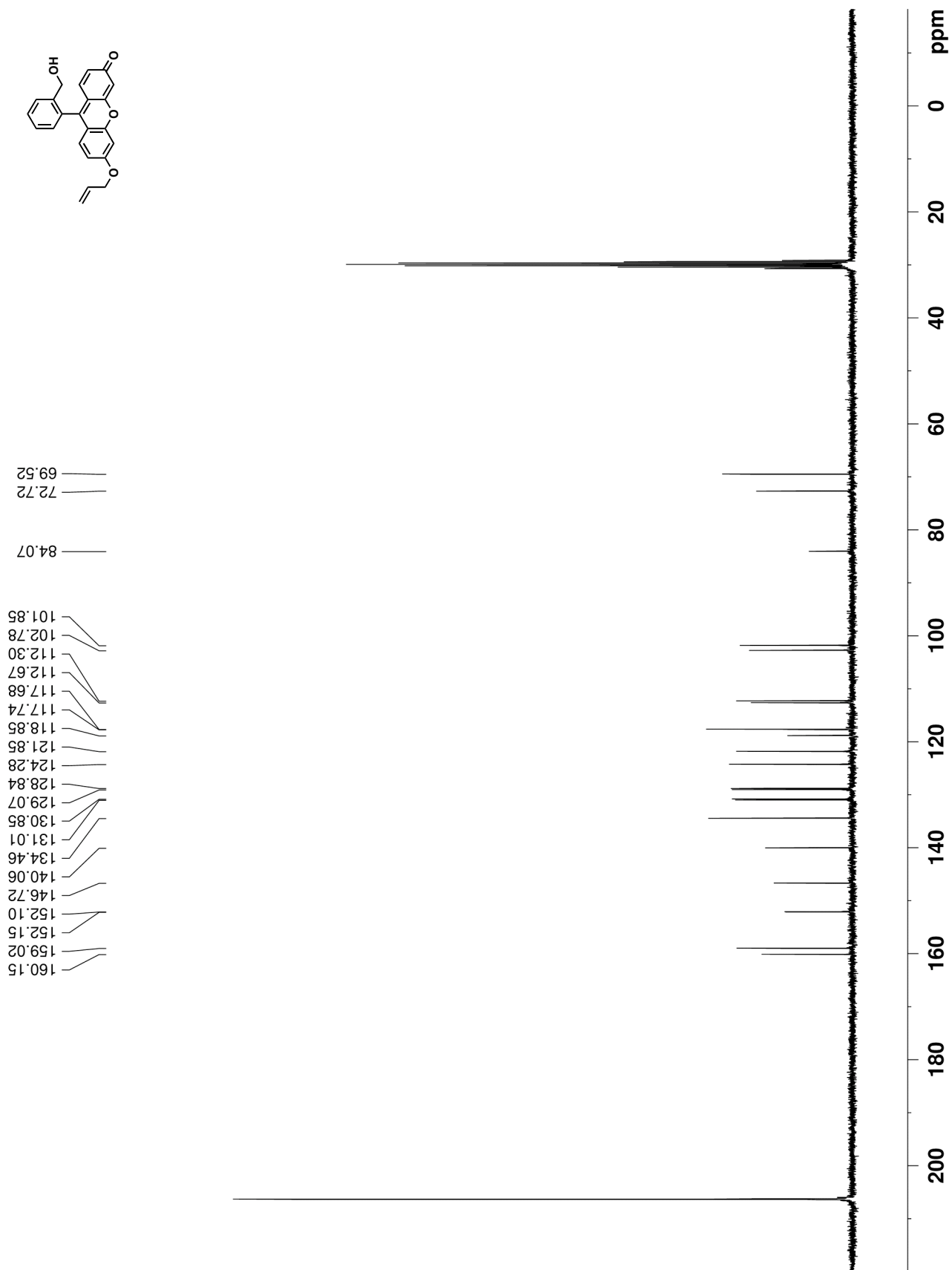
Figure S13. 13 C NMR spectrum of compound 11 (75 MHz, acetone- d 6 , 293K)
