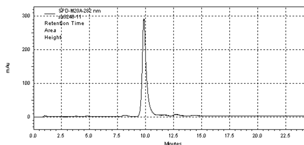
b) Compound 2
