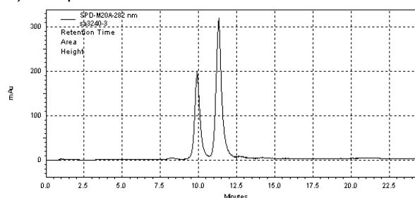
Figure S2. HPLC analysis of compound 3 . HPLC chromatogram of compound 3 (a), compound 2 (b), and a co-injected sample (c). HPLC analysis was performed on a Zorbax XDB C 18 column, 4.6 × 75 mm. Elution conditions: 1.0 mL/min, 60% MeOH/H 2 O to 100% MeOH/ H 2 O linear gradient elution from 0 to 20 min.
