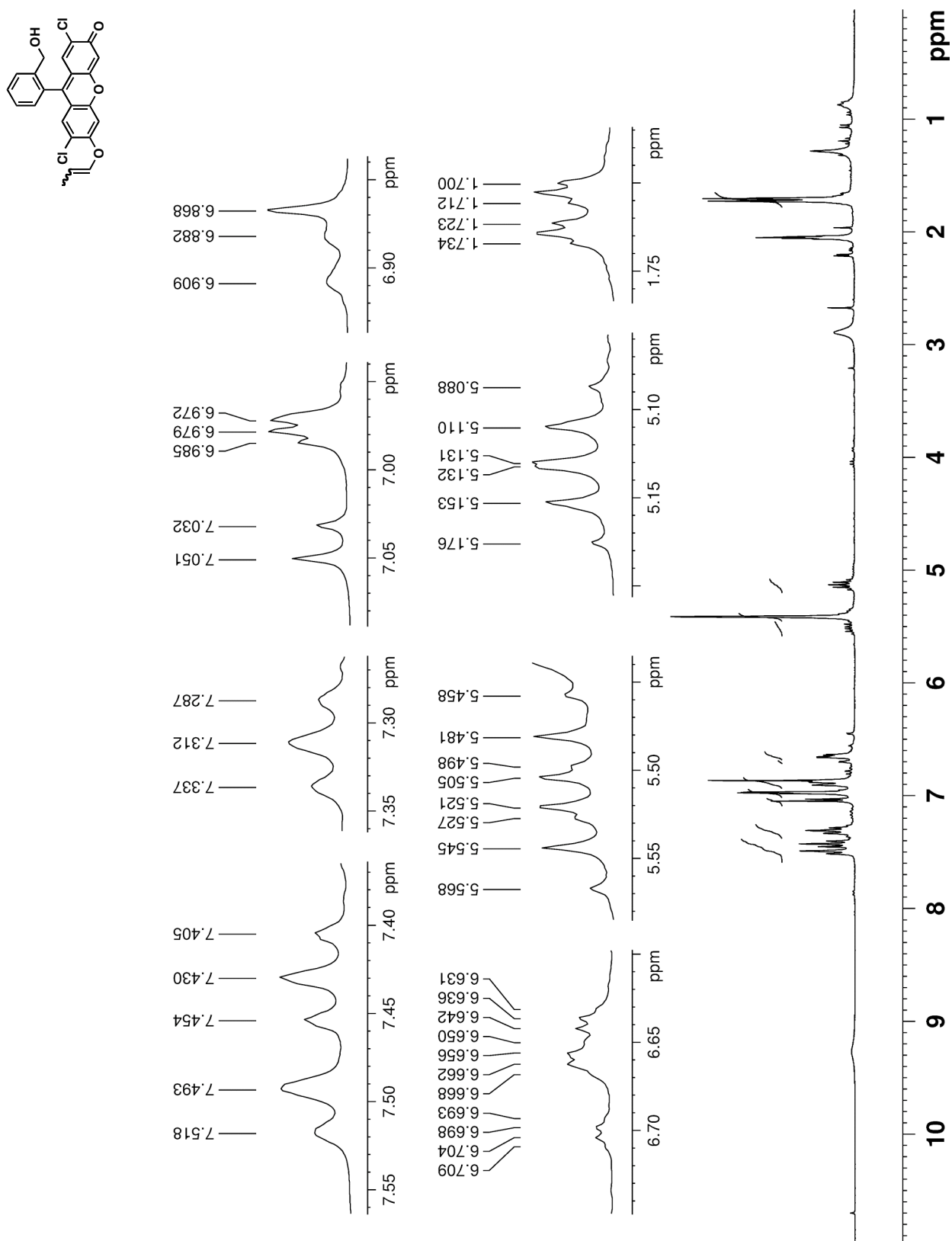
Figure S7. 1 H NMR spectrum of compound 3 (300 MHz, acetone- d 6 , 293K)
