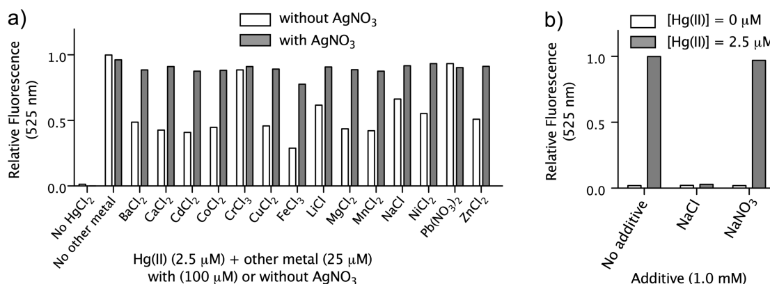
Figure 2. Compatibility of our method to detect Hg(II) in the presence of inorganic ions: (a) interference by inorganic materials ([HgCl 2 ] = 2.5 μM, [reagent shown] = 25 μM); (b) interference by NaCl but not by NaNO 3 . These experiments were performed in pH 4 buffer.
