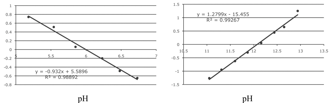
Figure S5. Analysis of the data in Figure 4a. The analysis was performed based on the following equation ( \text{pH} = \text{pK}_a - \log[(F_{\text{max}} - F)/(F - F_{\text{min}})] ). The \text{pK}_a values of compound 13 were 6.00 and 12.08.
