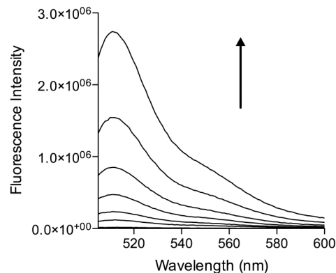
Figure S3. Fluorescence responses to Hg(II). The fluorescence response of 3 and 12 (Figures 1d and 4e) to various concentration of Hg was shown. [ 3 or 12 ] = 1.0 mM, [Hg] = 0, 1, 2, 4, 8, 16, 32 ppb.
