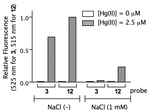
Figure S6. Hg detection in the presence of \text{Cl}^- in a pH 4 buffer.
