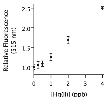
Figure 7. Application of 12 for the detection of Hg(II) in river water ( [12] = 1.0 \mu M ; [Hg(II)] = 0, 0.25, 0.5, 1, 2 , and 4 ppb; [AgNO_3] = 2.0 mM; 0.5% DMSO in 50 mM phthalate pH 4 water; 1 h; 25 °C). Titration of Hg(II) in river water was performed.
