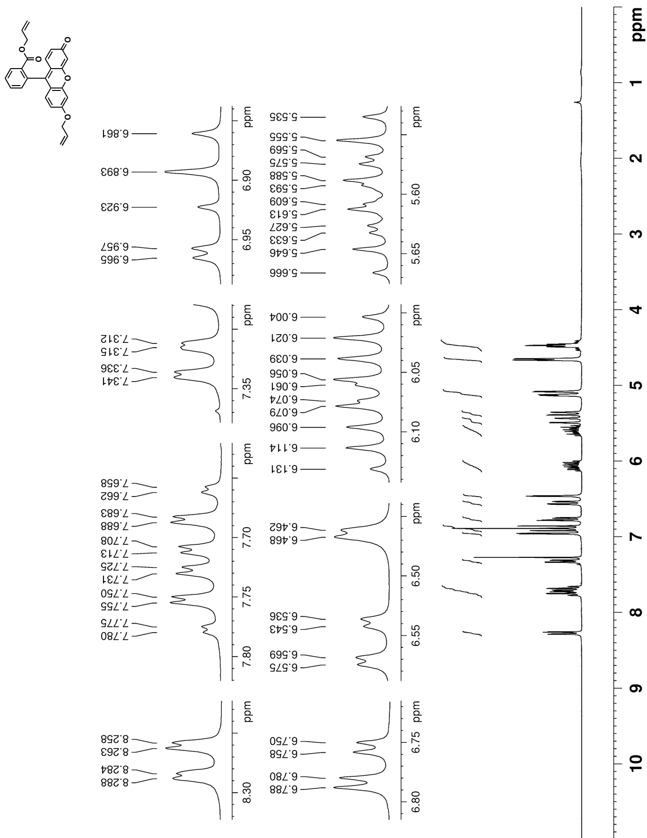
Figure S10. 1 H NMR spectrum of compound 10 (300 MHz, CDCl 3 , 293K)
