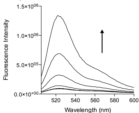
a) Compound 3
