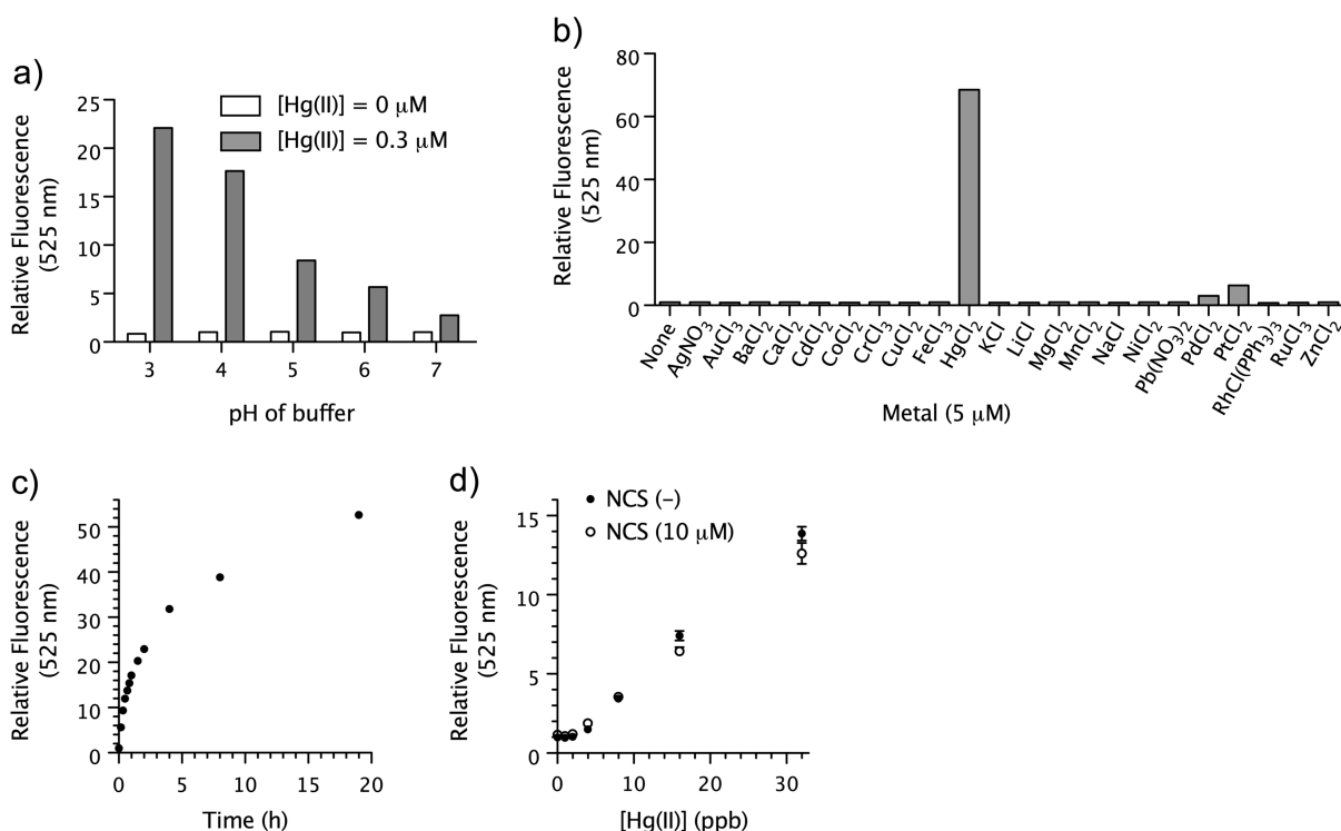
Figure 1. Conversion of 3 to 1 at 25 °C. [3] = 1.0 μM for all of the experiments. Except for (c), all of the reactions were performed for 1 h. Fluorescence intensities were measured after addition of 1.23 M phosphate pH 7 buffer. (a) pH dependence. (b) Metal selectivity in a 50 mM phthalate pH 4 buffer. Metal reagents: AgNO 3 , AuCl 3 , BaCl 2 , CaCl 2 , CdCl 2 ·2.5H 2 O, CoCl 2 , CrCl 3 , CuCl 2 ·2H 2 O, FeCl 3 , HgCl 2 , KCl, LiCl, MgCl 2 , MnCl 2 ·4H 2 O, NaCl, NiCl 2 , Pb(NO 3 ) 2 , Pd(NO 3 ) 2 , PtCl 2 , Rh(PPh 3 ) 3 , RuCl 3 , and ZnCl 2 . (c) Time course of the oxymercuration reaction: [Hg(II)] = 0.30 μM, 50 mM phthalate pH 4 buffer. (d) Correlation between fluorescence intensities and [Hg(II)] in the presence and absence of N -chlorosuccinimide (NCS). The experiments were performed in a 50 mM phthalate pH 4 buffer in triplicate. The graph shows the mean values and standard deviations.
