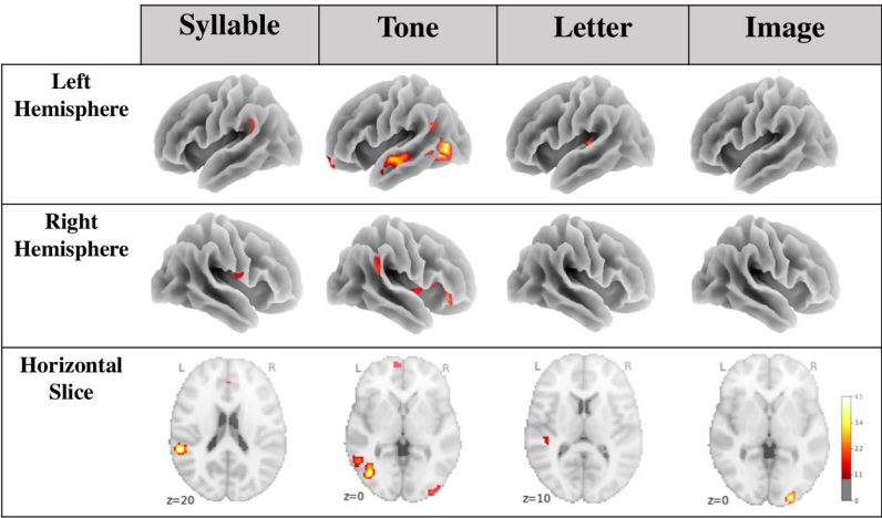
Figure 6: Neural activation at the group-level for structured blocks compared to random blocks within each modality and domain. Significant clusters were thresholded at voxel-level p < 0.001 and cluster-level p < 0.05 for each task. Horizontal slices were selected to depict the cluster with the maximum z-value. The color bar in the bottom, right corner reflects the same scale for all plots.
