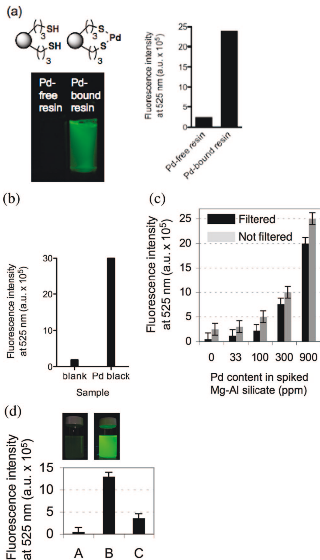
Figure 5. Pd detection in heterogeneous samples. [1] = 12.5 \mu M, [TFP] = 500 \mu M, and [NaBH 4 ] = 1.25 mM, and the assays were performed at 24 °C before fluorescence measurement. (a) Scavenger resin (Deloxan MP metal scavenger) and its Pd-bound form were treated with a solution of 1, NaBH 4 , and TFP in pH 7 buffer. (b) Detection in the presence of Pd black (<2.25 \mu mol/mL). (c) Detection in spiked Mg–Al silicate (Pd/Pt/Rh 2:2:1). Each reaction was quenched by the addition of N -acetylcysteine in large excess after 30 s and filtered before fluorescence measurement. Filtering of the samples, however, is not necessary for detection. (d) Detection in spent catalytic converter sample. A, Pd-free Mg–Al silicate; B, industry spent catalyst (alumina; [Pd] = 2345 ppm from ICP-MS); C, spent catalyst (cordierite; [Pd] = 1062 ppm, [Pt] = 827 ppm, [Rh] = 224 ppm from ICP-MS). Each reaction was quenched by the addition of N -acetylcysteine after 2 min and filtered before fluorescence measurement. Photos of samples A and B are shown above the graph.
