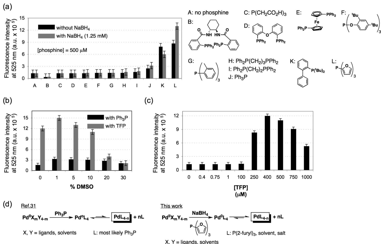
Figure 2. Phosphine screening and TFP optimization. [ 1 ] = 12.5 \mu M and [Pd] = 100 nM, and the assays were performed for 1 h at 24 ^{\circ} C in DMSO/pH 7 buffer (5:95 for (a) and (c)) before fluorescence measurement. (a) Phosphine screening. (b) Effect of % DMSO on phosphines with NaBH 4 . (c) Correlation between fluorescence intensity and [TFP]. (d) Conversion of all Pd II species to a uniform Pd 0 species.
