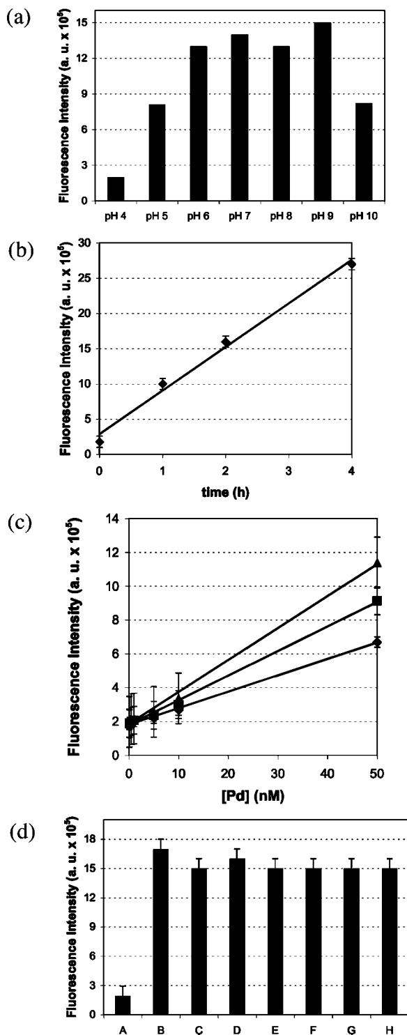
Figure 3. Catalytic Pd detection method with TFP/NaBH 4 . [1] = 12.5 \mu M, [TFP] = 500 \mu M, and [NaBH 4 ] = 1.25 mM, and the assays were performed for 1 h at 24 ^{\circ} C in DMSO/pH 7 buffer (5:95) before fluorescence measurement ( \lambda_{\text{em}} = 525 nm). (a) The pH-dependent deallylation of 1 in the presence of Pd (100 nM). (b) Initial rate analysis for deallylation of 1 in the presence of Pd (100 nM). y = 6.18x + 2.88 ; R^2 = 0.991 . (c) Correlation between fluorescence intensity and [Pd]. \blacklozenge = 1 h; y = 0.0971x + 1.81 ; R^2 = 0.998 . \blacksquare = 2 h; y = 0.145x + 1.81 ; R^2 = 0.997 . \blacktriangle = 4 h; y = 0.189x + 1.86 ; R^2 = 0.996 . (d) Fluorescence induction by various Pd species and oxidation states (100 nM): A, no Pd; B, PdCl 2 ; C, Pd(OAc) 2 ; D, Pd(acac) 2 ; E, Pd(PPh 3 ) 2 Cl 2 ; F, Pd(MeCN) 2 Cl 2 ; G, Pd 2 (dba) 3 ; H, Pd standard.
