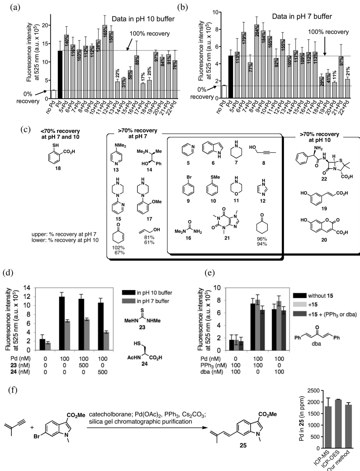
Figure 4. Pd detection in functionalized organic compound samples. [ 1 ] = 12.5 \mu M, [TfP] = 500 \mu M, and [NaBH 4 ] = 1.25 mM, and the assays were performed for 1 h at 24 ^{\circ} C before fluorescence measurement. (a) Detection in DMSO/pH 10 buffer (5:95) after pretreatment with concentrated HCl (60 mM) compared to a positive control (Pd). (b) Detection in DMSO/pH 7 buffer (150 mM) (5:95) after pretreatment with concentrated HCl (60 mM) compared to a positive control (Pd). (c) Structures of Pd-spiked compounds and summary of % recoveries. (d) Detection of Pd in the presence of 23 or 24 . (e) Detection of Pd in 15 in the presence of PPh 3 or dba. (f) Comparison of our method with other analytical methods. Compound 25 was prepared by a Pd-catalyzed reaction.
