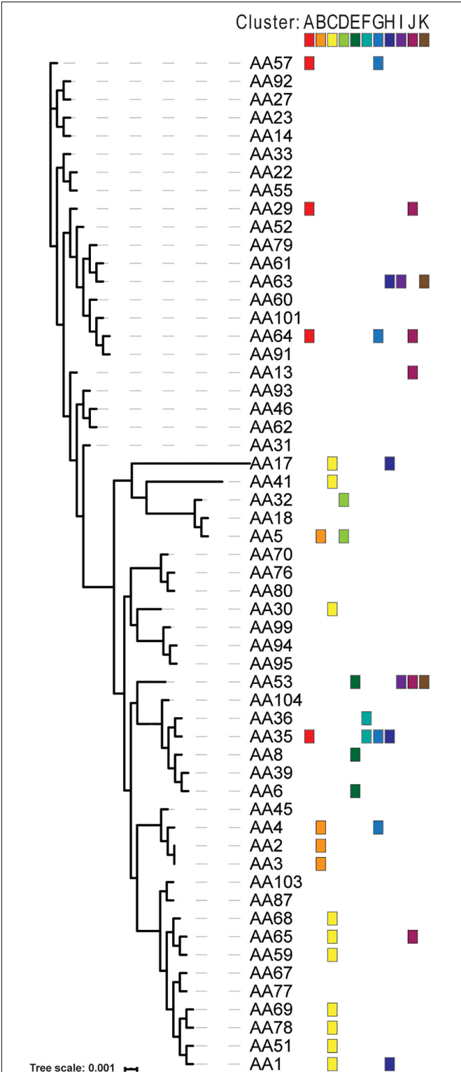
FIGURE 3 | Distribution of plasmid clusters across phylogenomic diversity of Egyptian S. aureus strains. The phylogenomic tree for the isolates was generated based upon the concatenated amino acid sequences of the single copy number genes in the core genome. The tree scale indicates the sequence divergence between the core genome sequence. The color blocks show the presence of a plasmid belonging to 1 of the 11 clusters.
