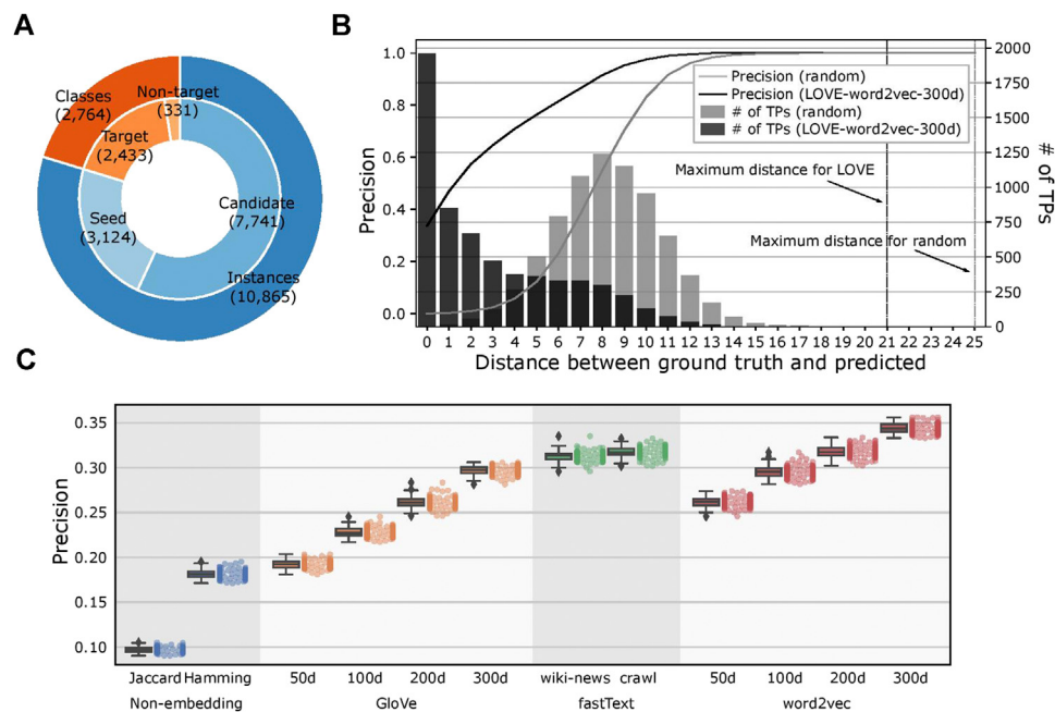
FIGURE 4 | Evaluation of the LOVE framework on a food ontology. (A) Number of ontology classes and food instances that were used for the LOVE-derived ontologies. Candidate instances are mapped to one of the target classes by LOVE, and each target class is initialized by seed instances. Classes without instances are not considered as target classes. (B) Distribution of precision and number of true positives of the mapped ontology as a function of shortest distance (hops) between the predicted class and the ground truth class for LOVE (black) and random assignment (gray) ( p value = 4.8 \times 10^{-102} ). (C) Precision of the ontology population for different similarity methods.
