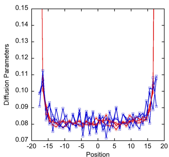
FIG. 5. Diffusion parameters \alpha (red circles) in the parallel direction and \beta (blue squares) in the perpendicular direction for the nonwetting system as a function of position z . The results of three independent simulations are shown.
