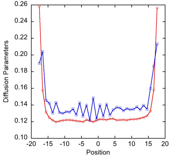
FIG. 11. Diffusion parameters \alpha (circles) and \beta (squares) for the nonwetting systems as a function of position from high sampling fits. Only the fit from a single simulation is shown.
