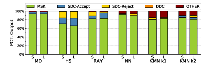
Fig. 8. Impact of Small and Large inputs on fault distribution.
