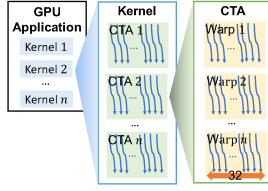
Fig. 2. A simplified overview of GPGPU application hierarchy.
