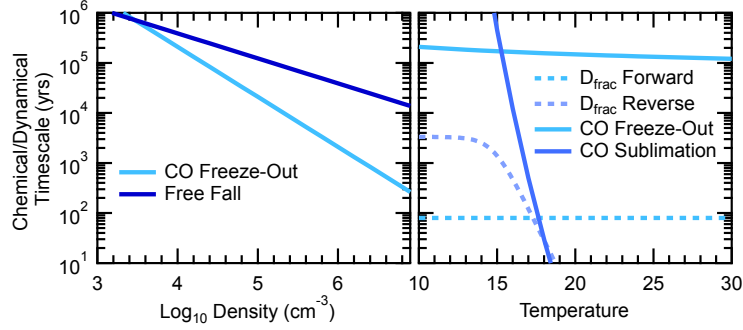
FIG. 11.— Chemical and dynamical timescales as a function of density (assuming T_{\text{gas}} = T_{\text{dust}} = 10 K), and temperature (assuming n_{\text{H}_2} = 10^4 \text{ cm}^{-3} ). CO freezeout using formalism of Hollenbach et al. (2009) and sublimation using the CO binding energy measured by Fayolle et al. (2014). For deuterium fractionation the timescales refer to the forward and reverse of the following reaction: \text{H}_3^+ + \text{HD} \leftrightarrow \text{H}_2\text{D}^+ + \text{H}_2 + 232 \text{ K} . We use the rates given by Hugo et al. (2009) and assume that the o/p ratio of the reactants and products are set by equilibrium at the specific temperature using the approximations described by Lee and Bergin (2015). Under these assumptions the reverse reaction begins to activate near 17 K, but this transition temperature will depend sensitively on the history of ortho and para \text{H}_2 during cloud and core formation (Flower et al. 2006; Pagani et al. 2013; Furuya et al. 2015).
