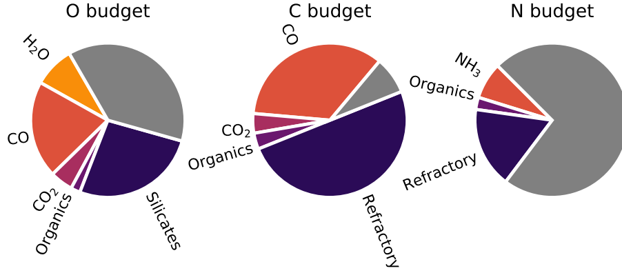
FIG. 9.— The O, C, and N budgets at the onset of star and planet formation, based on observations of ice abundances (Boogert et al. 2015), standard assumptions about CO, silicate and refractory carbon abundances, and solar system comet measurements of refractory nitrogen. Grey indicates an unknown component, which in the case of N is likely mainly N 2 , while the nature of the missing O carrier is unclear.
