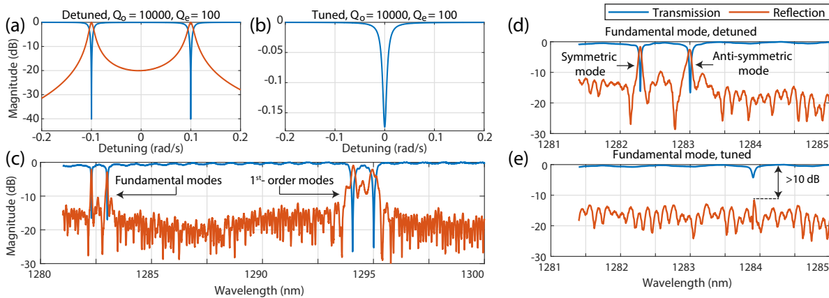
Fig. 2: (a) Response, given by CMT model, of detuned PhC nanobeam cavity strongly coupled to the input waveguide; (b) response (CMT model) after tuning the resonances; (c) experimental wide spectrum of detuned cavities showing the fundamental modes and the first-order modes; (d) spectrum around the fundamental modes before tuning, and (e) after tuning the symmetric cavity.
