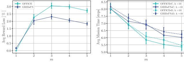
Fig. 6. Performance of distributed and centralized MILP approaches for OFFICE and GRID-FN, h = 10 . Left: Relative reward loss computed at t = 0 . Right: Average mission time. Bars show the std. error of the mean.
