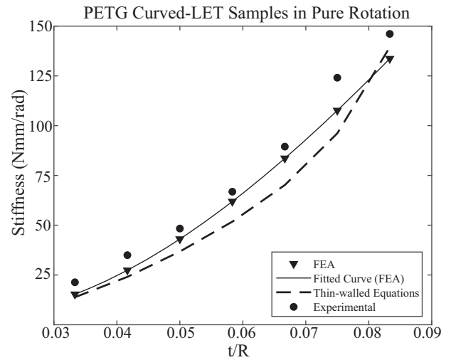
Fig. 12 Comparison of experimentally derived 3D printed curved LET joint stiffness to FEA and thin-walled LET models
