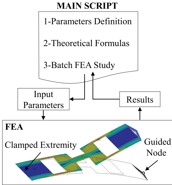
Fig. 9 Schematic of the software framework
