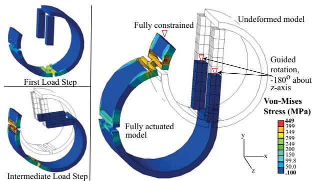
Fig. 14 FEA results of the expanding cylinder mechanisms with LET joints in Nitinol
