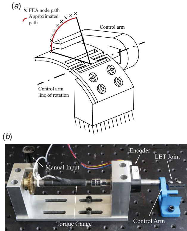
Fig. 11 Physical prototyping of the curved LET joint: (a) schematic showing the deflection path of the LET joint and (b) experimental setup
