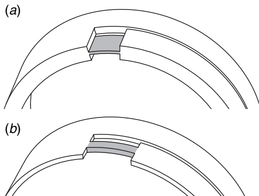
Fig. 4 (a) The wall thickness reduction method (reduces h in beam) for creating SLFPs or pre-curved flexures and (b) the width reduction method (reduces w in beam), which is only viable when the cylinder wall thickness is less than the beam width
