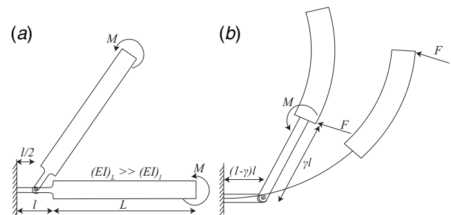
Fig. 2 (a) PRBM for a SLFP and (b) PRBM for an initially curved beam
