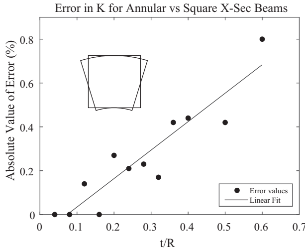
Fig. 7 Plot showing relative error between torsional constants of annular cross section and rectangular cross section beams. The finite mesh used to obtain annular torsional constants may account for the non-smooth pattern from low to high t/R ratio.
