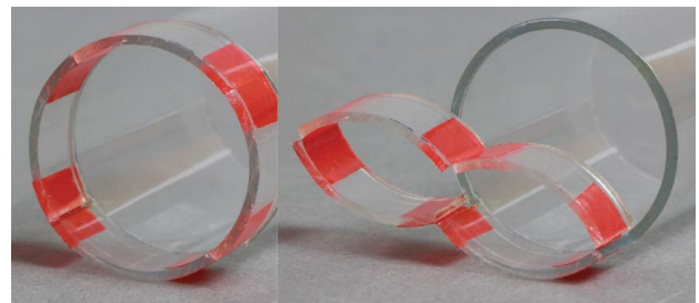
Fig. 5 Parallel guiding cylindrical DM with membrane joints. The cylinder is 38 mm diameter polycarbonate tubing, cut on an Epilog M2 CO2 laser cutter, and the membrane is red acrylic tape.
