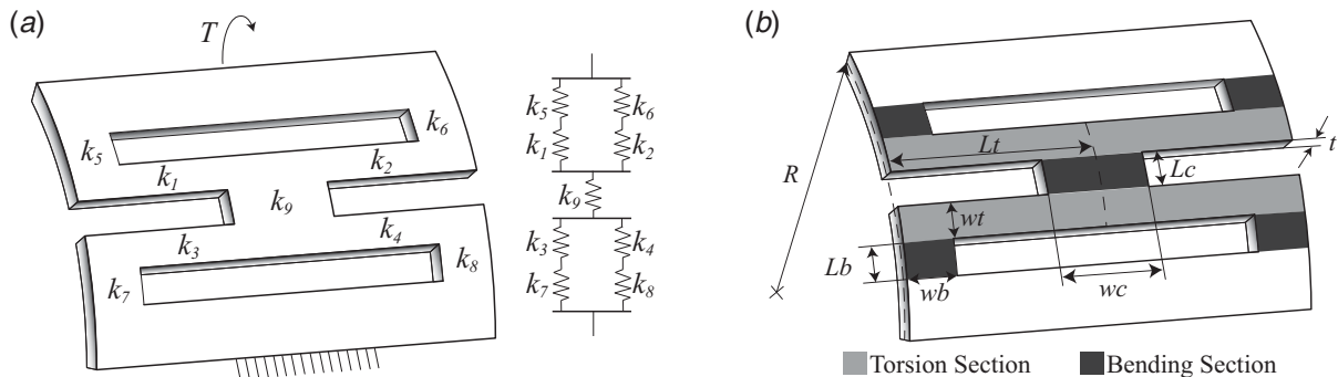
Fig. 8 Schematic describing parameters used in the MATLAB analysis and elsewhere in this paper: (a) Spring diagram for the inside LET joint and (b) principal dimensions for the inside LET joint
