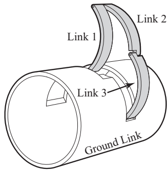
Fig. 1 An example cylindrical DM. Links 1, 2, and 3 are highlighted, and the ground link is the cylinder body.
