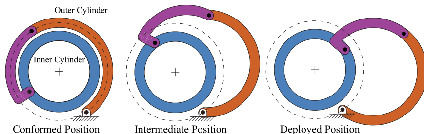
Fig. 13 Functional schematic of the multiplying cylinder mechanism
