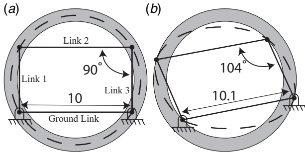
Fig. 6 (a) Skeleton diagram showing a parallel guiding mechanism aligned to a reference surface (dotted line) in the middle of the cylinder walls. (b) The same parallel guiding mechanism, with the same link lengths, but with joints aligned with the inner or outer surface of the cylinder.
