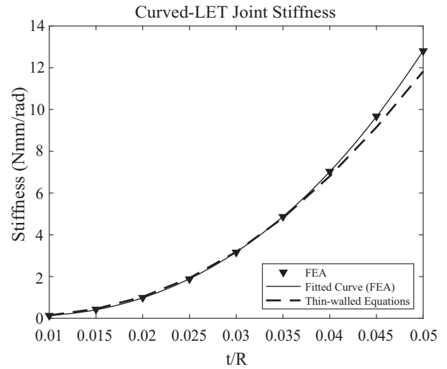
Fig. 10 Curved LET joint stiffness comparison between FEA and thin-walled assumption models
