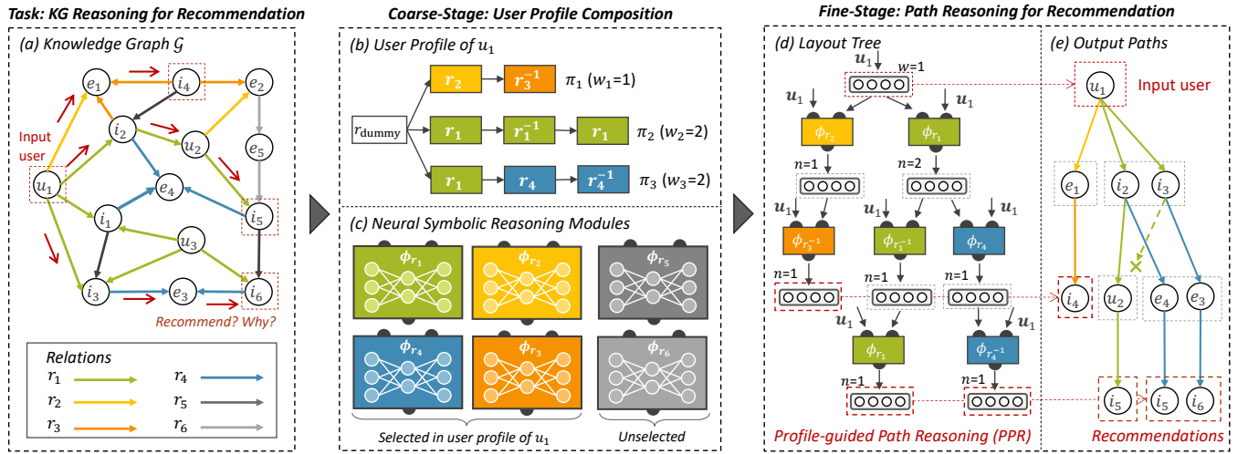
Figure 2: Illustration of CAGE , a coarse-to-fine KG reasoning approach. (a) Given a KG and a start user, the goal is to conduct multi-step path reasoning to derive recommendations. (b) In the coarse stage, a personalized user profile is constructed based on historic user behavior in the KG. (c) To make use of the user profile in path reasoning, an inventory of neural symbolic reasoning modules is maintained. (d) In the fine stage, a layout tree is composed with the modules based on the user profile, which is exploited by the proposed PPR algorithm (Alg. 1) to produce (e) a batch of paths along with recommendations.
