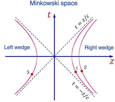
FIG. 1. Trajectory of atoms uniformly accelerated in different Rindler wedges.
