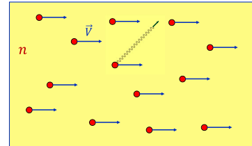
FIG. 3. Ensemble of atoms moving through a medium with an equal velocity V > c/n and emitting Cherenkov radiation.
