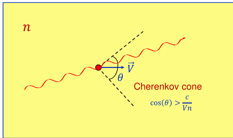
FIG. 2. A ground-state atom is moving through a medium with a constant velocity V > c/n . Photon propagating in the direction inside the Cherenkov cone \cos \theta > c/Vn cannot be absorbed by the atom.
