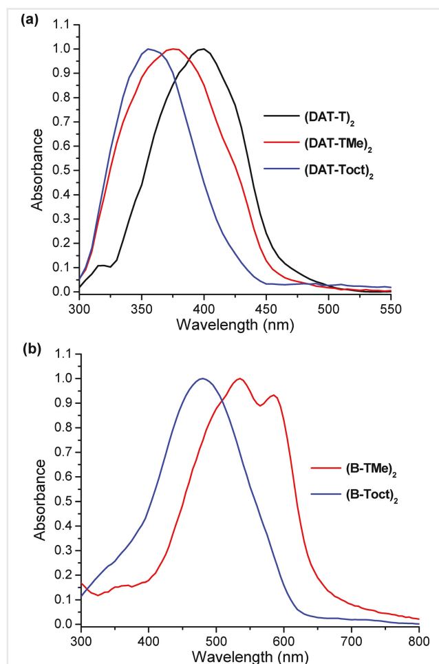
Figure 5 Normalized thin-film absorbance spectra for (a) (DAT-T) 2 , (DAT-TMe) 2 , and (DAT-Toct) 2 ; (b) (B-TMe) 2 and (B-Toct) 2 .
