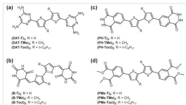
Figure 3 Molecular representations of the simple ditopic systems studied in this work based on (a) diaminotriazine (DAT), (b) barbiturate (B), and (c) phthalhydrazide HB-capable units (PH), and (d) phthalic ester HB-incapable units (PMe).
