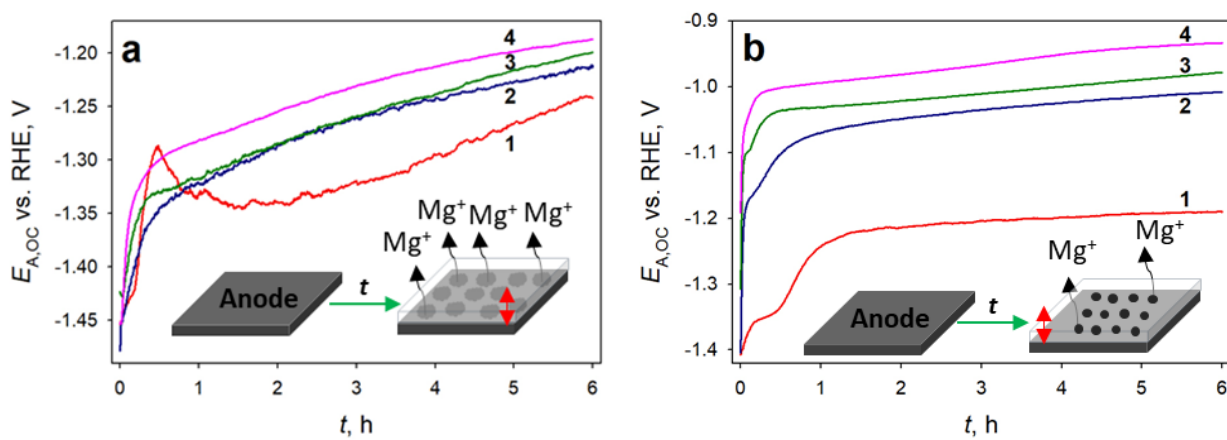
Figure 2. Anodic OCP curves obtained with (a) pure Mg and (b) AZ31 Mg alloy anodes in various concentrations of aqueous ammonium dihydrogen phosphate: (1) 7.7, (2) 77, (3) 150, and (4) 300 mM, respectively.
