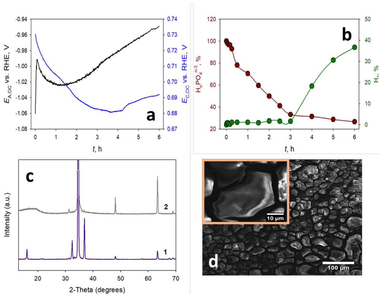
Figure 12. (a) Anodic/cathodic OCP curves obtained for the reactor with pure Mg and 316SS plates. (b) Phosphate removal and di-hydrogen production over time in a poultry wastewater sample. (c) XRD spectra of the struvite formed in (1) synthetic and (2) poultry wastewaters samples, respectively. (d) SEM image obtained of the struvite layer produced on the anode in a poultry wastewater sample. Inset: High resolution SEM image.
