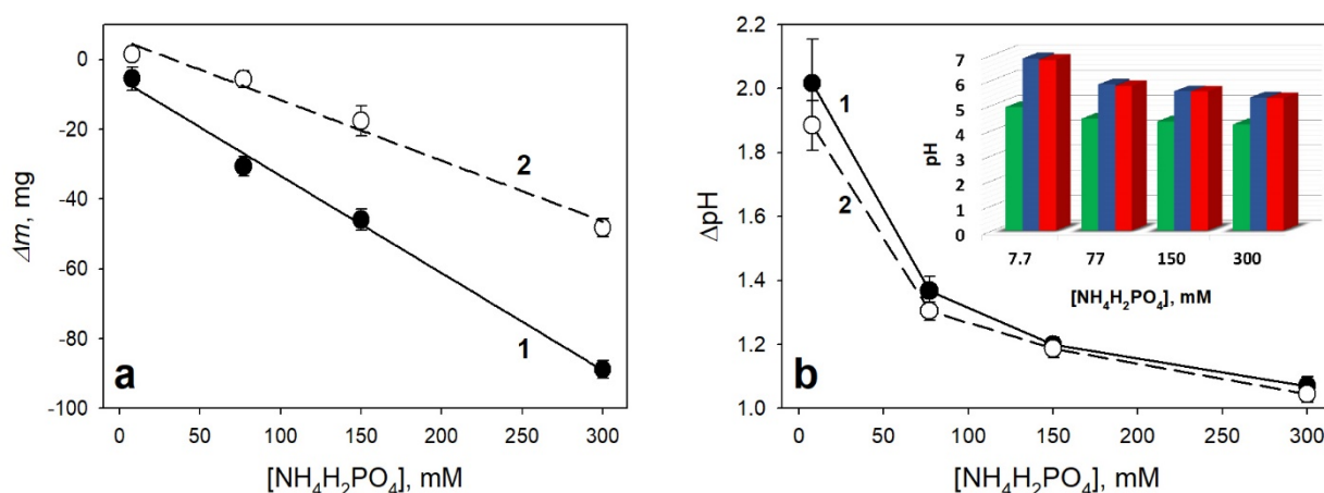
Figure 8. (a) The anode mass losses due to Mg oxidation of the (1) pure Mg and (2) AZ31 Mg alloy plates during the 6-hour OCP measurements. Mass losses are reported as absolute values. (b) pH difference in the bulk solution for various ammonium dihydrogen phosphate concentrations for reactors containing (1) pure Mg and (2) AZ31 Mg alloy as anodes. Inset: the initial pH of the bulk solution (green), the final pH of the bulk solution after 6-hour OCP measurements in case of pure Mg (blue) and AZ31 Mg (red) in various concentrations of the test solution. The reported values represent the average results from four separate experiments ( n=4 ) and the error bars the standard deviation.
