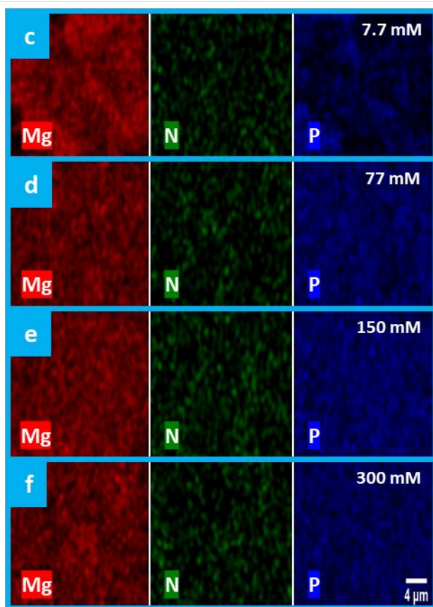
Figure 5. The element atomic percentages (At%) of the struvite layers obtained with the reactor containing the (a) pure Mg; and (b) AZ31 Mg alloy anodes, respectively. The corresponding EDX elemental maps of Mg, N and P for the struvite obtained with the reactor containing (c-f) pure Mg anode; (g-f) AZ31 Mg alloy anode, in various concentrations of the test solution.
