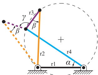
Fig. 7 Class 2 mechanism in its crossed (solid), conformed (dashed) and open (dotted) configuration
