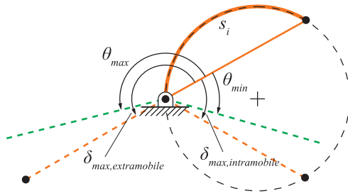
Fig. 14 It is possible for the limits of a link's motion to occur prior to \delta
