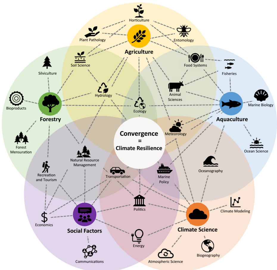
Fig. 1 Convergence research framework illustrating disciplines connected to climate resilience in agriculture, forestry, and aquaculture
