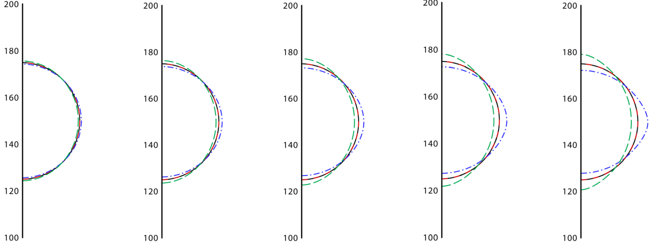
FIG. 3. Moving bubble in a uniform vertical flow. Model A is shown with a black solid line (circular shape in the center), and model B is shown with a red dashed line (circular shape in the center). Models A and B are on top of each other. Model C is shown with a blue dash-dot-dot line (horizontal elliptical shape), and model D is shown with a green long-dashed line (vertical elliptical shape). Pe = 20 . Left to right is t = 5T_f , t = 10T_f , t = 15T_f , t = 20T_f , and t = 25T_f .
