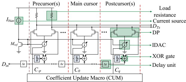
Fig. 3. Schematic of a feed-forward equalizer (FFE) architecture.
