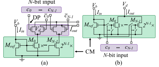
Fig. 1. Schematic of a (a) current-steering DAC, (b) current-switching DAC.
