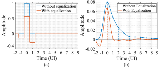
Fig. 2. An unequalized pulse with its precursor and postcursor, and its equalized output. The signal is sampled at integer multiples of the unit interval (UI), and the equalized signal provides low ISI at t \leq -1 and t \geq 1 .
