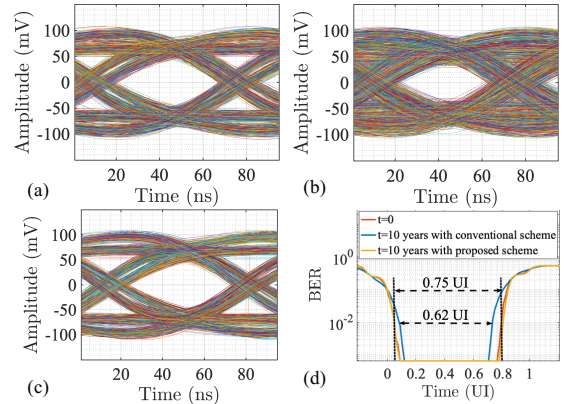
Fig. 9. Aging effects on eye diagram of HSLs: (a) at t = 0 , (b) at t = 10 years with the conventional scheme, (c) at t = 10 years with the proposed scheme, (d) bathtub curve comparison in unit interval (UI).
