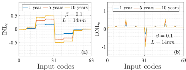
Fig. 7. Impact of aging on the main cursor of the FFE: (a) INL, (b) DNL.
