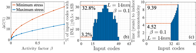
Fig. 6. Aging effects on 6-bit IDAC. Aging can (a) increase gain error, (b) increase INL, (c) induce non-monotonicity.
