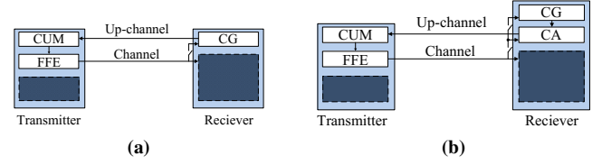
Fig. 4. (a) Conventional communication between Tx and Rx for the FFE. (b) Aging mitigation scheme with CA unit on the Rx side.
