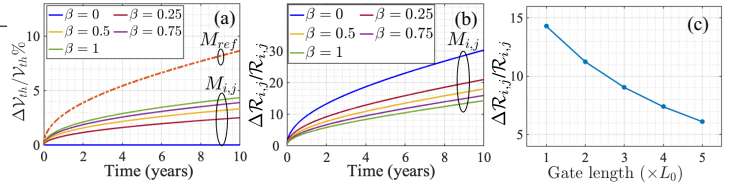
Fig. 5. (a) V_{th} degradation of M_{ref} and M_{i,j} due to aging with varying \beta . (b) Change in transfer ratio of M_{i,j} due to aging with varying \beta . (c) Change in transfer ratio of M_{i,j} with varying gate length, L .
