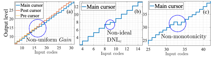
Fig. 8. Segments of the transfer curves that illustrate (a) non-idealities in Gain G , (b) non-idealities in DNL, and (c) nonmonotonicity.
