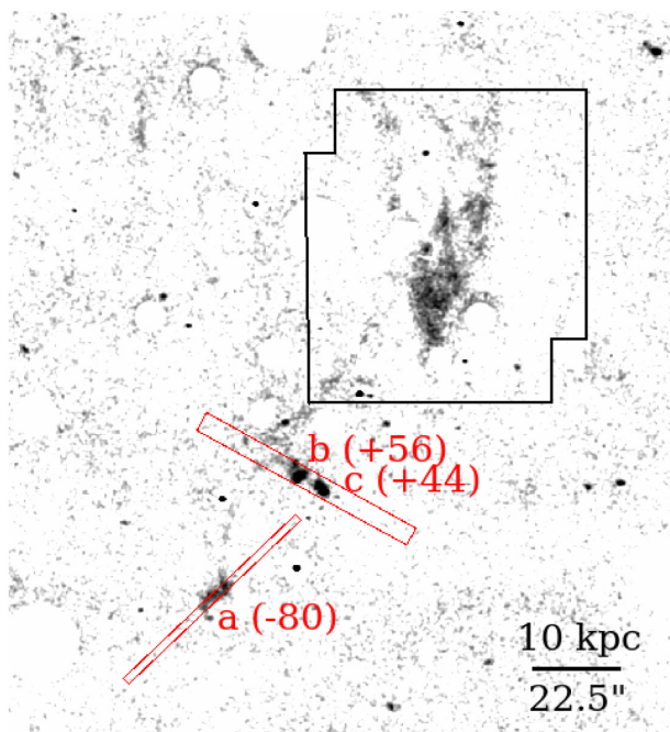
Figure 6. The APODIS slit positions at the southeast of the H\alpha OC. The velocities (in a unit of \text{km s}^{-1} , relative to z = 0.024 as in Fig. 3) are also shown. The image shows the net H\alpha emission from Subaru , with stars and galaxies masked out. The MUSE FOV is also shown in a black solid box.
