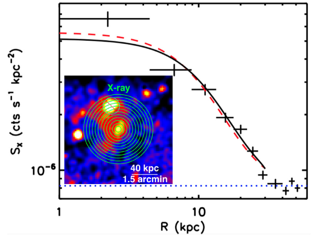
Figure 4. The SBP of the OC. The solid black line is the best fit of a \beta -model convolved with the XMM PSF, while the dashed red line is the \beta -model without correction for the PSF. The dotted blue line is the local background level. The inset in the left corner shows the annuli for the SBP extraction. The annuli are centred on the X-ray peak.
