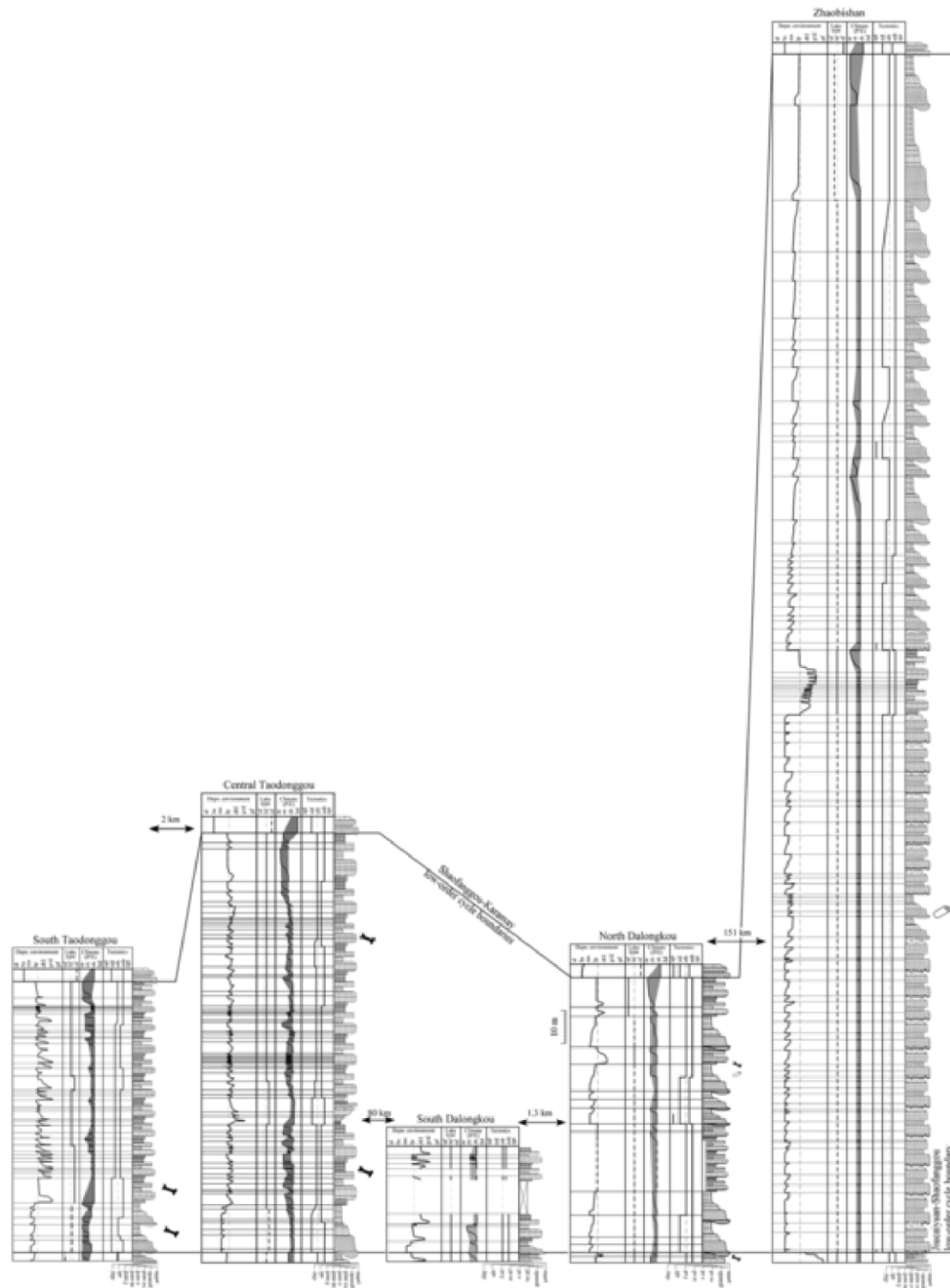
Fig. 12. Stratigraphic correlation of lower the Olenekian Shaofanggou low-order cycle, showing 1–100-km variability in depositional environment, lake type, and climatic and tectonic conditions. Occurrences of some permineralized wood and vertebrate fossils are marked. The base of Shaofanggou low-order cycle is the correlation datum. See Figs. 6–9 for individual simplified sections, Figs. 1 and S1–S4 for locations and detailed stratigraphy of individual sections, and Fig. 4 for explanations.
