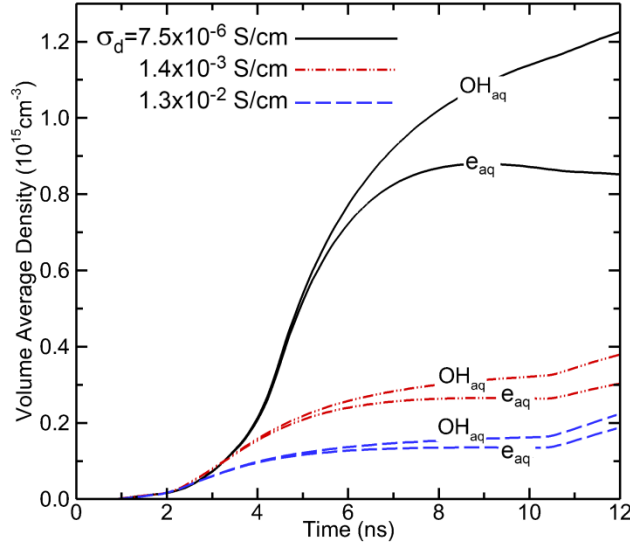
Figure 10 - Densities of solvated electrons ( e_{\text{aq}} ) and \text{OH}_{\text{aq}} for values of the conductivity of the droplet, \sigma_d of 7.5 \times 10^{-6} S/cm, 1.4 \times 10^{-3} S/cm and 1.3 \times 10^{-2} S/cm.
