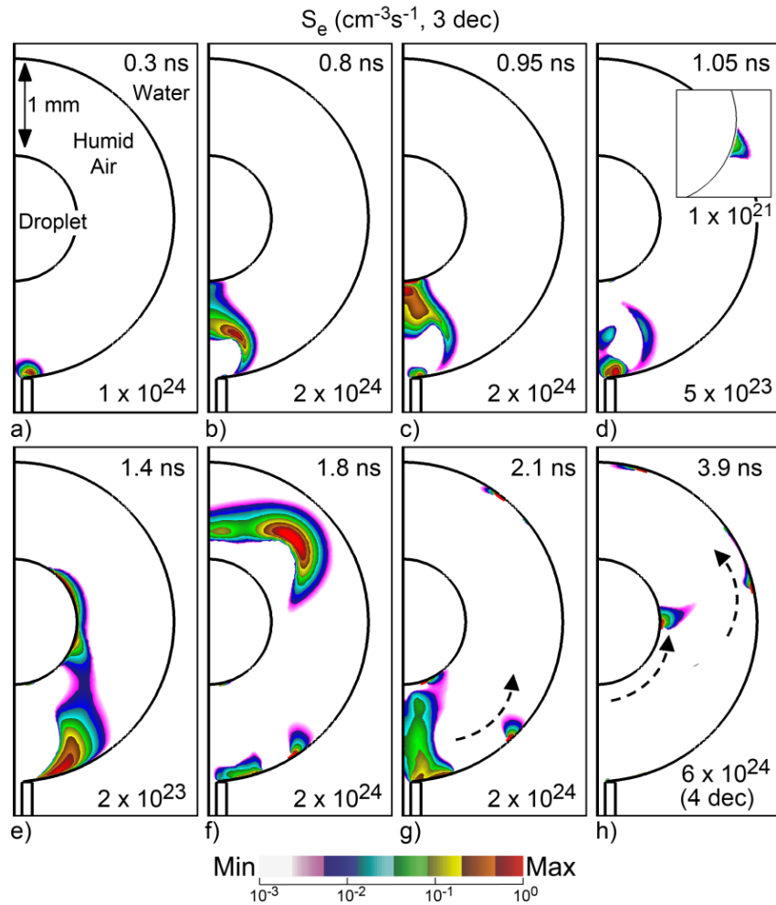
Figure 4 - Electron impact ionization source ( S_e , in \log_{10} scale over 3 decades unless otherwise noted) for the base case at a) 0.3 ns, b) 0.8 ns, c) 0.95 ns, d) 1.05 ns, e) 1.4 ns, f) 1.8 ns, g) 2.1 ns and h) 3.9 ns. The maximum value shown in each frame. The embedded image in d) shows a 100-times-intensity enhanced view. The arrows in h) indicate the direction of propagation tracks of surface discharges.
