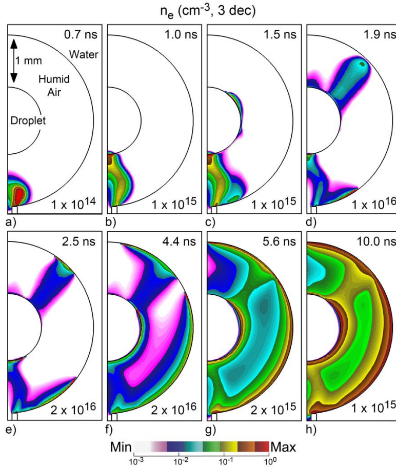
Figure 3 - Electron density ( n_e , in \log_{10} scale over 3 decades) for the base case at a) 0.7 ns, b) 1.0 ns, c) 1.5 ns, d) 1.9 ns, e) 2.5 ns, f) 4.4 ns, g) 5.6 ns and h) 10.0 ns. The maximum is value shown in each frame.
