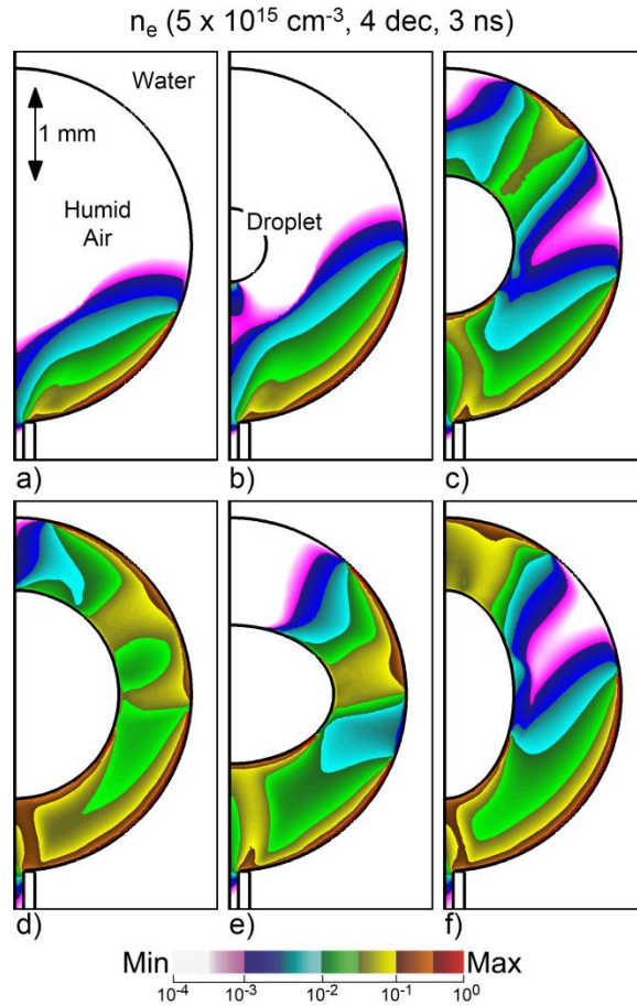
Figure 13 - Electron density (4 decade \log_{10} scale) in the bubble at 3.0 for different sizes and shapes of the droplets. The shapes of the droplets are described by, for example, 0.5x-1.0y, indicating that the x axis has a length 0.5 that of the base case and the y axis has a length equal to the base case. a) no droplet. b) 0.5x-0.5y, c) 1x-1y (base case), d) 1.5x-1.5y, e) 1.5x-1.0y, and f) 1x-1.5y.
