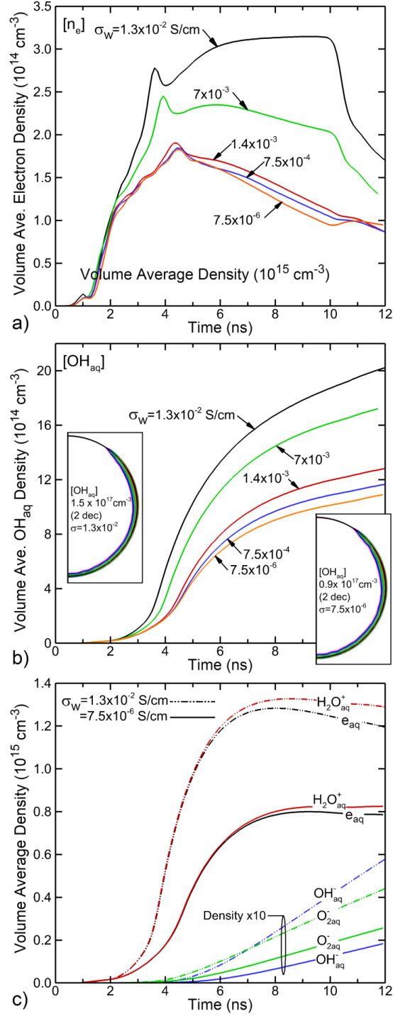
Figure 8 - Plasma properties for different values of the conductivity of the water surrounding the bubble, \sigma_w . (a) Volume-averaged electron density in the air. (b) \text{OH}_{\text{aq}} in the water droplet. (c) Density of aqueous ions and electrons for \sigma_w = 1.3 \times 10^{-2} \text{ S/cm} and 7.5 \times 10^{-6} \text{ S/cm} . The other conditions are identical with those in the base case. The embedded images in (b) show the spatial distribution of \text{OH}_{\text{aq}} density at 10 ns for \sigma_w being 1.3 \times 10^{-2} \text{ S/cm} and 7.5 \times 10^{-6} \text{ S/cm} .
