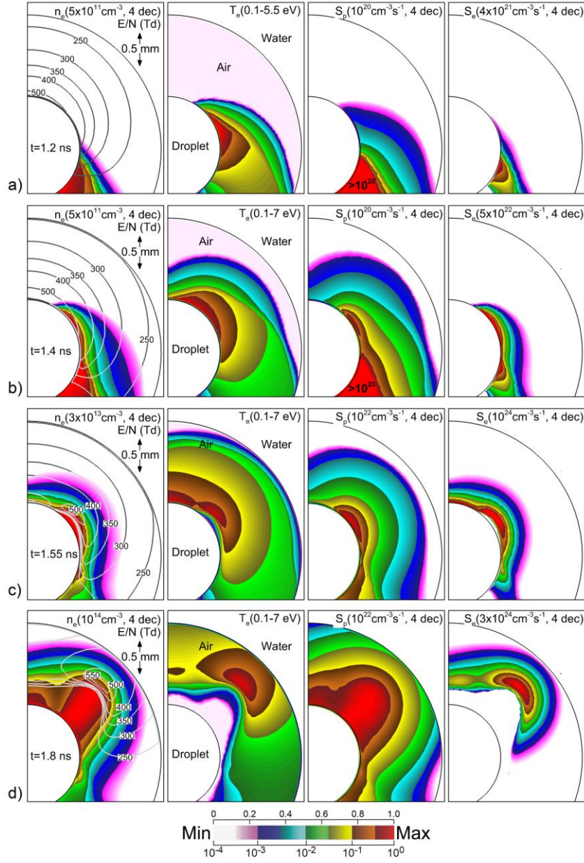
Figure 6 - Plasma properties as the secondary streamer is launched at (a) 1.2 ns, (b) 1.4 ns, (c) 1.55 ns and (d) 1.8 ns. From left to right at each time are the electron density ( n_e , flood) and reduced electric field ( E/N , contours), electron temperature ( T_e ), photoionization rate ( S_p ), electron-impact ionization rate ( S_e ). The maximum value for log plots or range of values for linear plots are noted in each frame. The contours for E/N are labeled in units of Td ( 1 \text{ Td} = 10^{-17} \text{ V-cm}^2 ).
