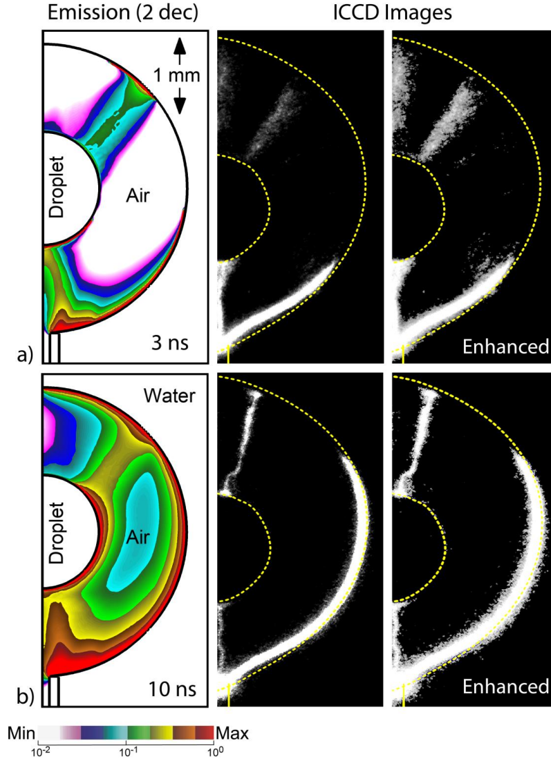
Figure 11 - Comparison of simulated optical emission and experimental observations a) early and b) late during the voltage pulse. The simulated emission is represented by time integrated emission from excited states of N_2 , H, OH, O and O_2 . The corresponding ICCD images had a 5 ns gate. The conductivity of both the water droplet and the surrounding water is 1.3 \times 10^{-2} S/cm. Two versions of the ICCD images are shown – actual data and artificially enhanced to show more detail.
