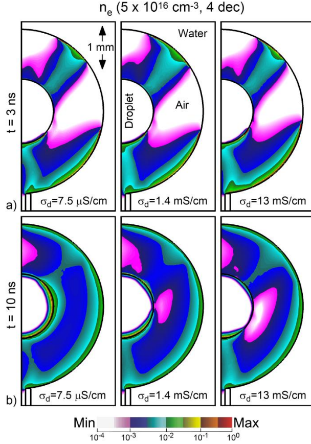
Figure 9 - Densities of the sum of gas and liquid phase electrons ( n_e ) at (a) 3.0 ns and (b) 10.0 ns for the conductivity of the droplet ( \sigma_d ) being 7.5 \times 10^{-6} \text{ S/cm} , 1.4 \times 10^{-3} \text{ S/cm} , and 1.3 \times 10^{-2} \text{ S/cm} . The other conditions are the same as the base case.
