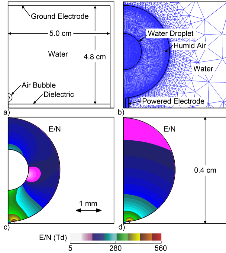
Figure 1- Schematic of the model. a) Entire computational domain. b) Enlarged view of the plasma region (air bubble and water droplet) and the unstructured mesh. c) Spatial distribution of reduced electric field E/N without plasma (applied voltage 20 kV). d) E/N without water droplet.
