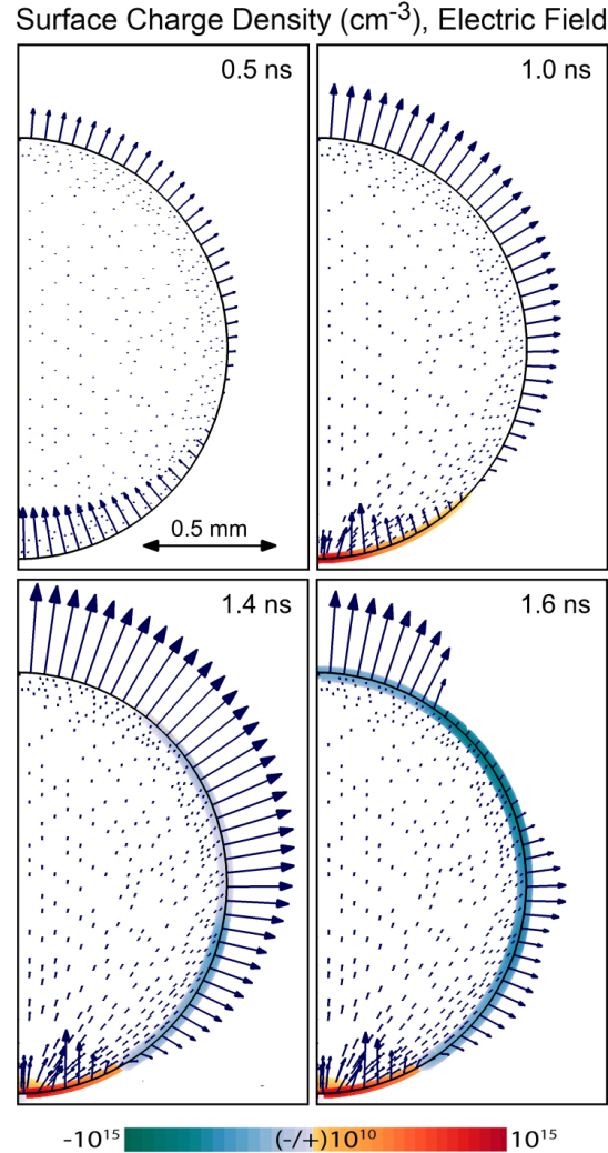
Figure 5 - Surface charge density and electric field vectors in the water droplet at 0.5, 1.0, 1.4 and 1.6 ns. The length of the electric field vector is proportional to the local electric field strength.
