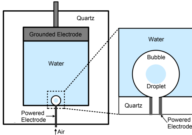
Figure 2 - Schematic of experimental setup.
