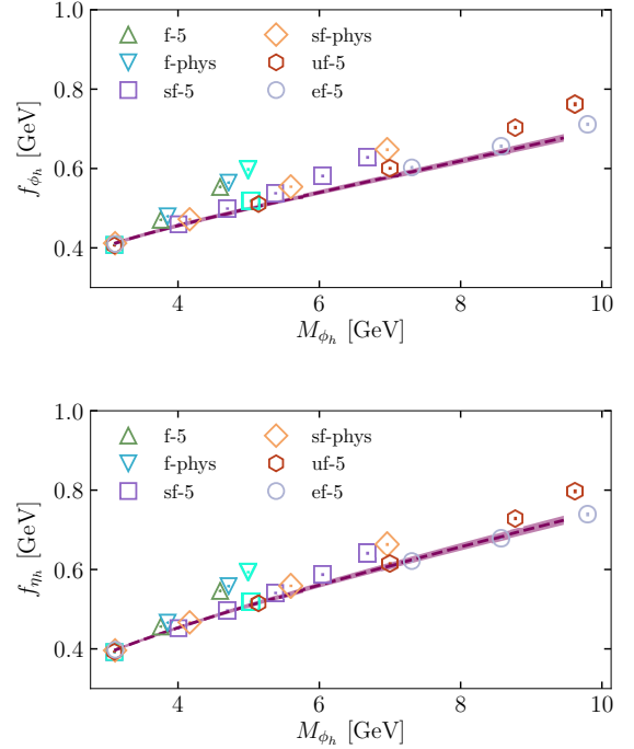
FIG. 4. Upper panel: The \phi_h decay constant plotted against the \phi_h mass. The symbols correspond to different gluon field ensembles, as given in the legend (see Table I for a list). Points including quenched QED are shown in cyan, indistinguishable from pure QCD points underneath. The dashed line and error band show the fit described in the text evaluated at zero lattice spacing and physical sea quark masses. Lower panel: The \eta_h decay constant plotted against the \phi_h mass, symbols and fit line as above.
