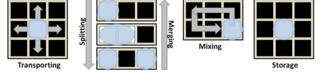
(b) The DMFB ISA supports five basic operations: transporting, merging, splitting, mixing and storage, in addition to I/O on the perimeter of the array.
