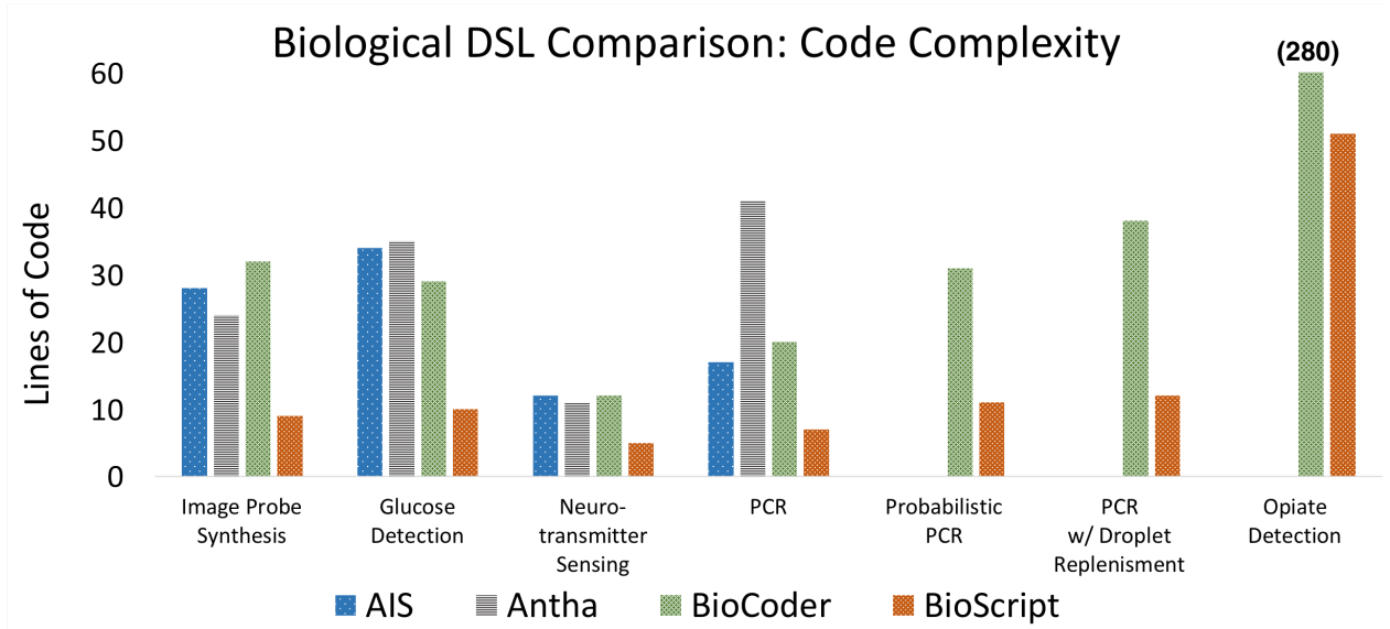
Figure 7: The number of lines of code to specify Image Probe Synthesis, Glucose Detection, Neurotransmitter Sensing, PCR, Probabilistic PCR, PCR w/ Droplet Replacement, and Opiate Detection in AIS, BioCoder, Antha, and BioScript . We were unable to specify the latter three assays in AIS and Antha.
