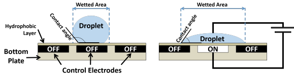
(a) The electrowetting principle [10, 13]: applying an electrostatic potential to a droplet at rest reduces the contact angle with the surface, thereby increasing the surface area in contact with the droplet
