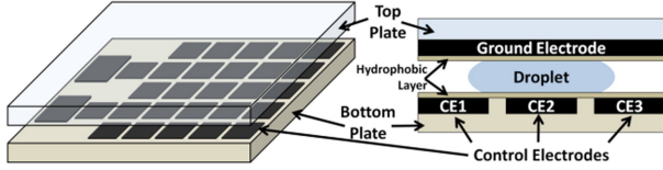
(a) Left: A DMFB is a planar array of electrodes [15]. Right: Cross-sectional view.
