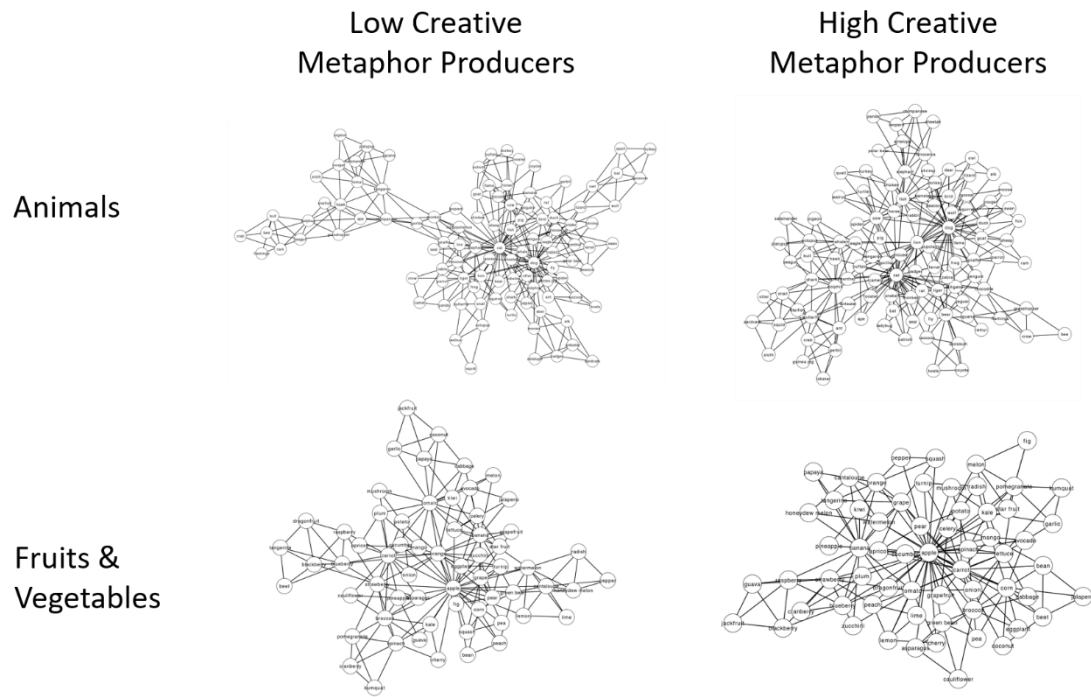
Figure 2. A 2D visualization of the semantic network of high and low creative metaphor producing groups for two semantic categories
