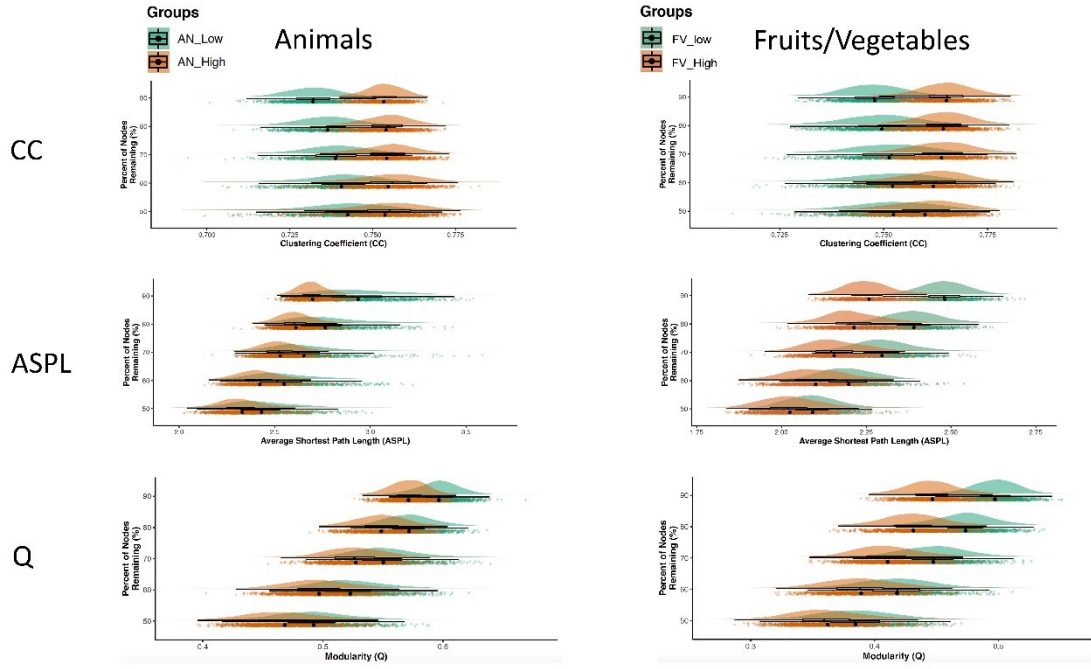
Figure 3. Plots of the bootstrapped partial network measures (1000 samples per nodes remaining percentage). Density plots are above the scatterplots (individual dots depict a single sample), with a black dot representing the mean. The y-axis denotes the percentage of nodes remaining (e.g., 90% = 90% nodes remaining in the bootstrapped sample). The x-axis denotes the network measure values.
