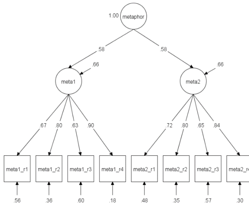
Figure 1. Confirmatory factor analysis of creative metaphor. Factor scores were extracted to form high and low metaphor groups for group-based semantic network analysis. meta1 = boring class metaphor; meta2 = gross food metaphor; r1-r4 = rater1-rater4.
