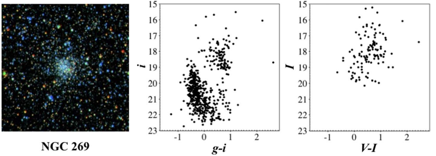
Figure 7. Cluster NGC 269 in the SMC. Left: SMASH gri color image, middle: SMASH CMD, and right: MCPS CMD.
