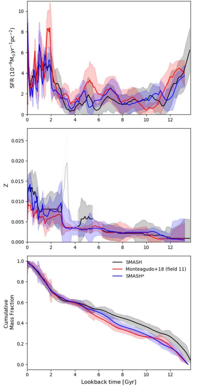
Figure 6. Comparison between the star formation histories computed using SMASH and VIMOS (Monteagudo et al. 2018) data. We show the star formation rate as a function of time (top), the chemical enrichment (middle), and the cumulative mass fraction (bottom). We compare three different solutions: SMASH (black) using SMASH data and the set of parameters that better suits the data, Monteagudo+18 (field 11, red), and SMASH* (blue) using SMASH data and mimicking the input parameters used in Monteagudo et al. (2018). The middle panel shows with transparency the age range where a small fraction of stars has been found and thus, where a fully reliable metallicity determination is hindered. Shaded regions represent uncertainties in the SFH recovery computed as described in Hidalgo et al. (2011).
