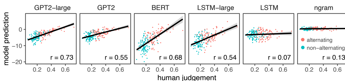
Figure 3: Spearman correlation between human judgment and model prediction, across 200 verbs. Judgments were averaged across themes and recipients, hence the lower overall preferences for the double-object.
